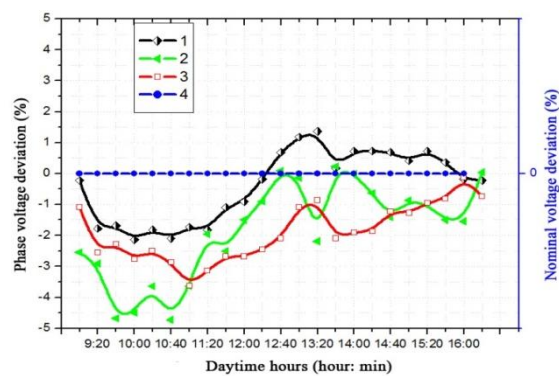
Fig.3. Dependence of the voltage deviation of each phase and the deviation of the nominal voltage from the day time of day (26.12.2019). 1-First phase voltage deviation; 2- second phase voltage deviation; 3- third phase voltage deviation; 4- rated voltage deviation.
