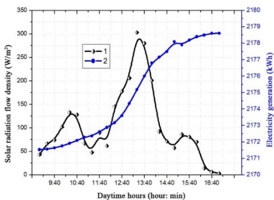
Fig.6. Dependence of solar radiation flow and electricity production of PPS on daytime (07.01.2020) 1-dependence of solar radiation flux density on the day time of day; 2 -generation of PPS electricity from the daytime.
