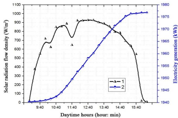
Fig.4. Dependence of the solar radiation flow and electricity production of the PPS on the time of day (26.12.2019)
