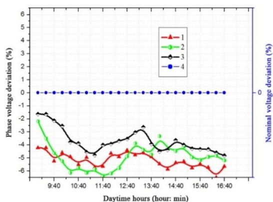
Fig.5. Dependence of the voltage deviation of each phase and the deviation of the nominal voltage from the day time of day (07.01.2020). 1- first phase voltage deviation; 2- second phase voltage deviation; 3- third phase voltage deviation; 4- rated voltage deviation.
