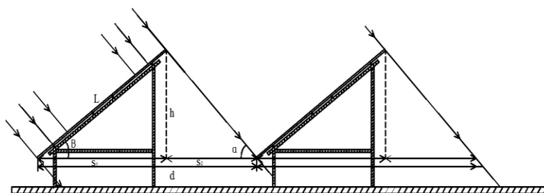
Fig.2. Determining the optimal distance between the rows of PVB
