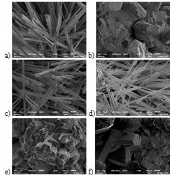
Fig. 2. Electron microphotographs of the synthesized crystals of the calcium sulfate dihydrate: a) no additive; b) with SMF additive; c) with MC additive; d) with VAEVC additive; e) with SMF + VAEVC additive; f) with SMF + MC additive.
