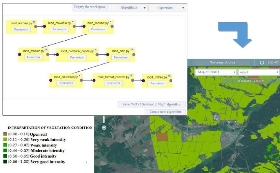
Fig. 2. Algorithmic structure for the monitoring of the grain culture condition and the results of one of its cycles
