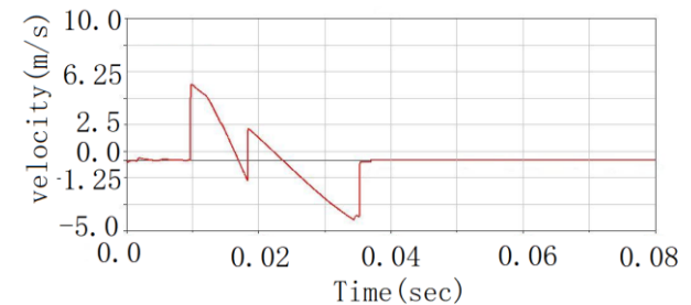
Figure 10. Curve of balancer speed
