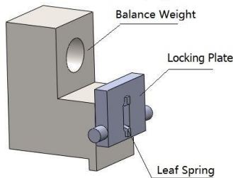
Figure 2. Assembly diagram of balance weight and locking plate
