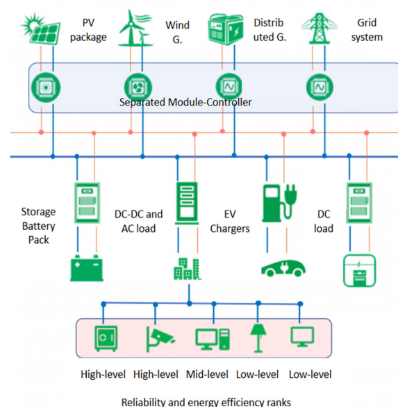
Fig. 1. Schematic form of a typical local energy internet
