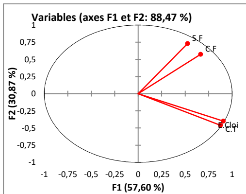
Fig. 2. Representation of the variables according to the factorial plane F1 and F2 inside the correlation circle.
