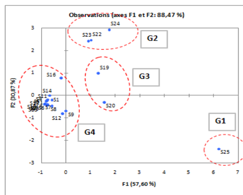
Fig. 5. Representation of sampling sites on factorial plane F1 and F2
