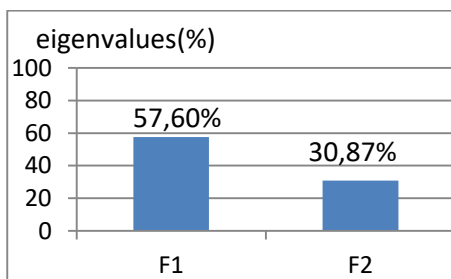
Fig. 3. Representation of the factors F1 and F2 based on the eigenvalues
