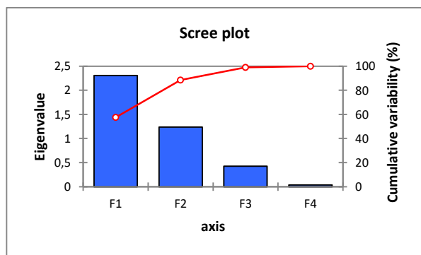
Fig. 4. PCA graphical approach: Representation of cumulative variability of the PCA axis
