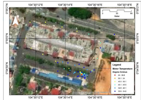
Fig. 9. Field test location and motor temperature record coordinate.
