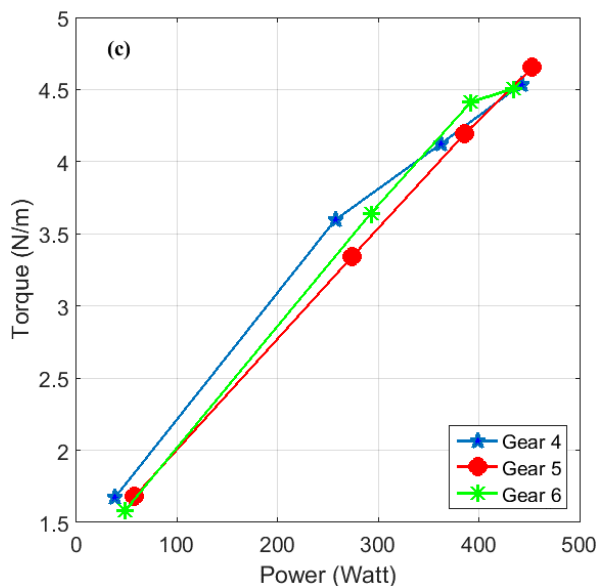
Fig. 8. Results of power compared to torque in different gear and percentage handle throttle.
