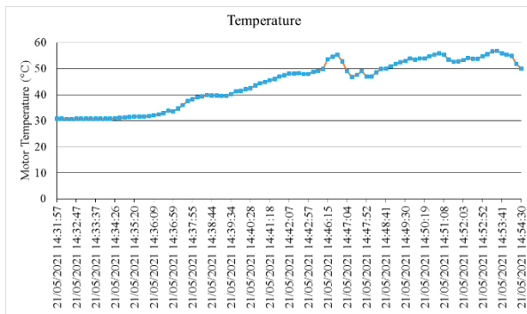
Fig. 12. Motor temperature record based time riding.
