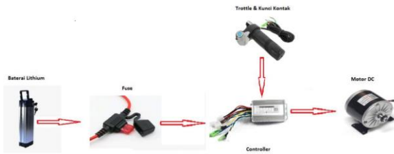
Fig. 2. E-bike component configuration in this prototype.
