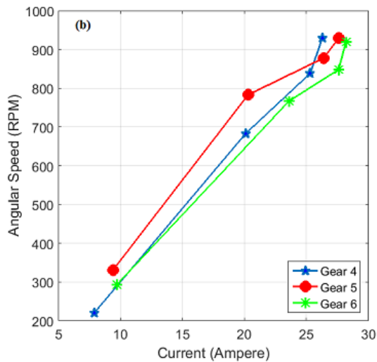
Fig. 7. Results of electrical current measurement compared to angular speed in different gear and percentage handle throttle.
