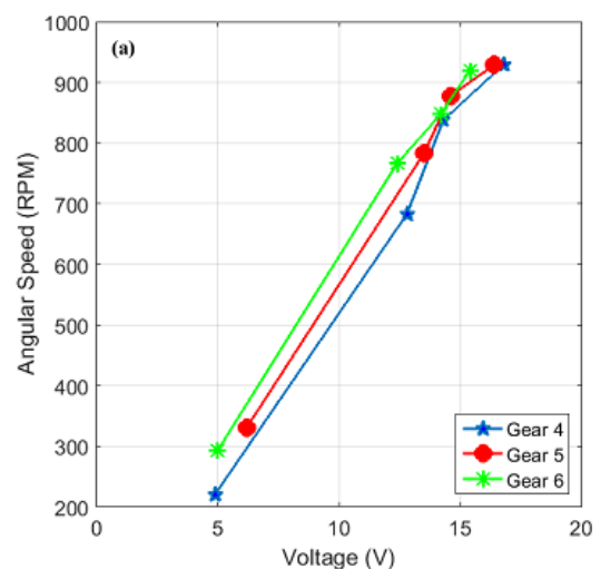
Fig. 6. Results of voltage measurement compared to angular speed in different gear and percentage handle throttle.
