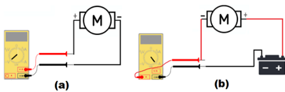
Fig. 4. Illustration voltage (a) and current (b) measurement using a multimeter.
