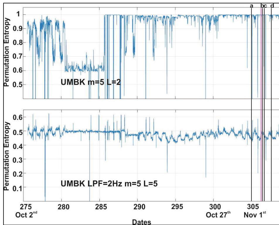
Fig. 5. PE graphs from UMBK station. Top : PE graph from combination m = 5 and L = 2 without filtering step. Bottom : PE graph from combination m = 5 and L = 5 using filtered data LPF 2 Hz.
