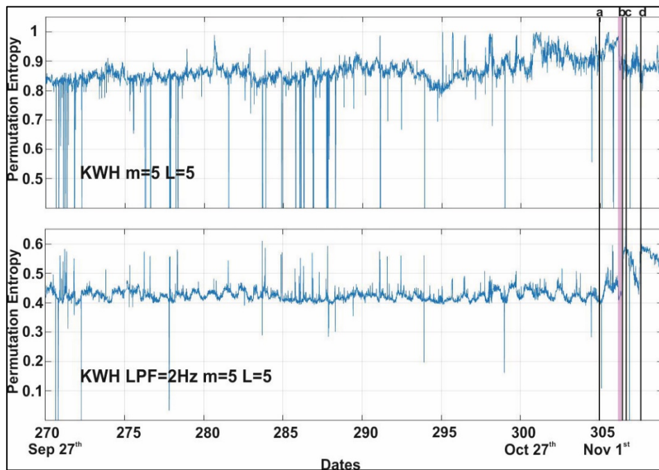
Fig. 4. PE graphs from KWH station that situated inside the crater. Top : PE graph from combination m=5 and L=5 without filtering step. Bottom : PE graph from combination m = 5 and L = 5 using filtered data LPF 2 Hz.
