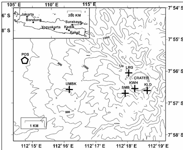
Fig. 2. Location map of Kelud volcano seismic stations and observation post. KWH = Kawah; KLD = Kelud; LRG = Lirang; SMB = Sumbing; UMBK = Umbuk; POS = observation post [7].
