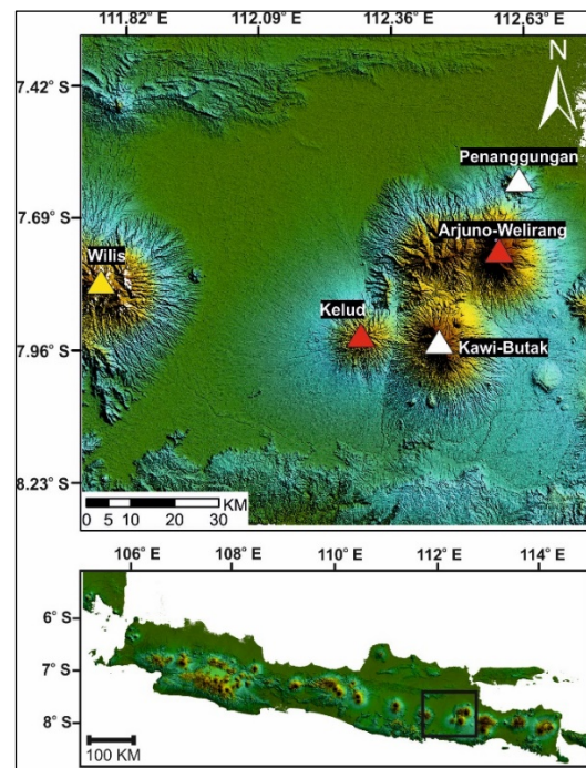
Fig. 1. Location map of Kelud volcano and its surroundings. Red – yellow – white triangles show volcano type A – B – C. Inset map shows volcanoes distribution at Java Island.
