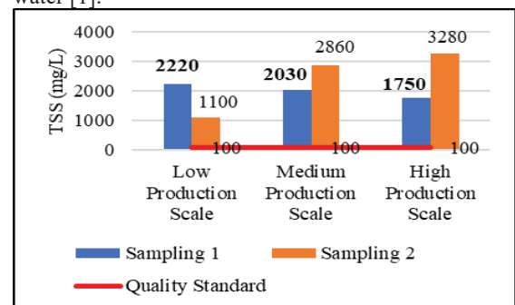
Fig. 8. Total suspended solids (TSS) of the liquid waste by-products of the tofu industry during low, medium and high production scales
