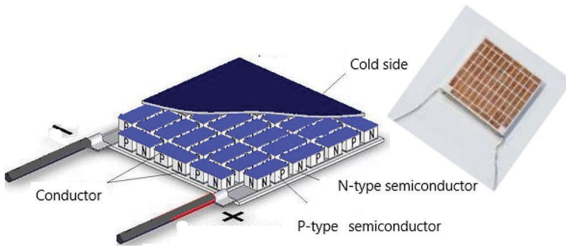
Fig. 2. Peltier element
