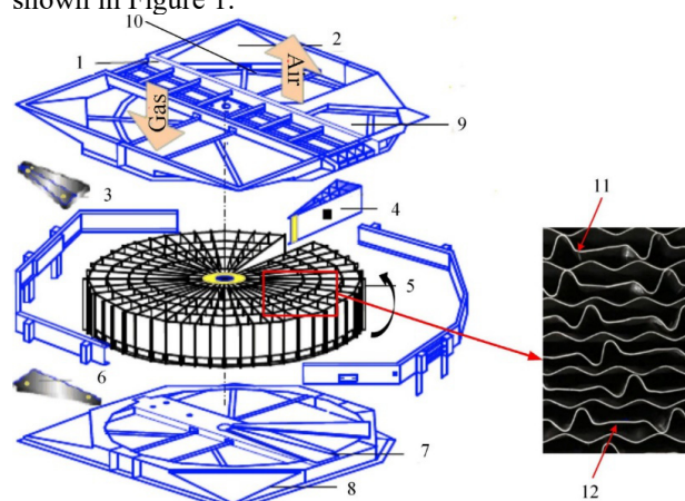
(1. Upper beam; 2. Upper gas channel; 3. Hot end sector seal; 4. Segmented steel plate; 5. Corrugated plate; 6. Cold end sector seal; 7. Lower beam 8. Bottom flue gas channel; 9. One time Air outlet; 10. Secondary air outlet; 11. Corrugated board; 12. Positioning board)
