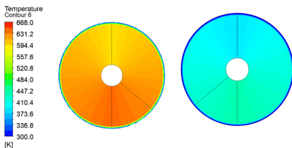
Fig. 3. Temperature distribution diagram of the hot end and the hot end of the air preheater
