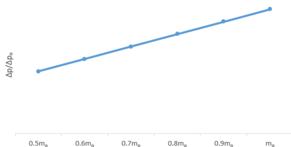
Fig. 4. The influence of mass flow on pressure drop of preheater
