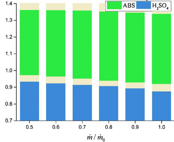
Fig. 5. The influence of mass flow rate on cold end corrosion and ABS deposition distribution
