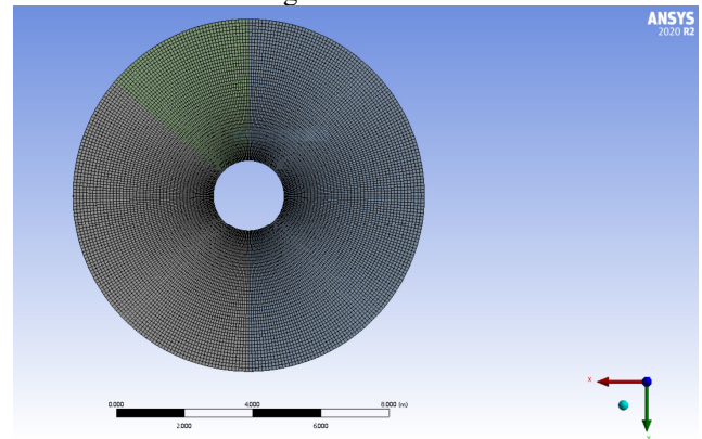
Fig. 2. Schematic diagram of grid division of air pre-heater
