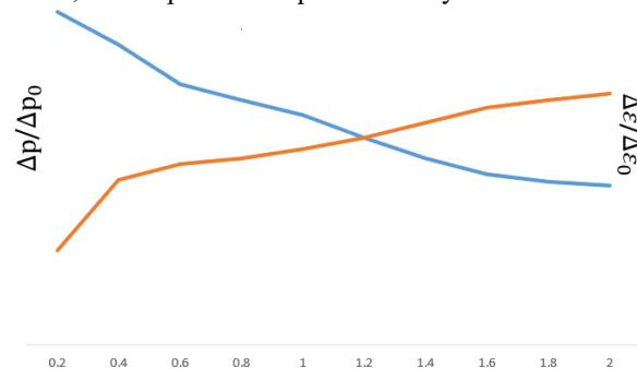
Fig.6. The effect of speed on the efficiency and pressure drop of the preheater
