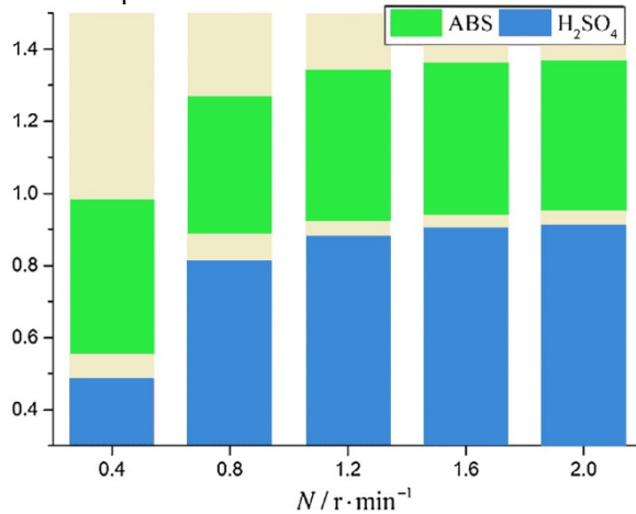
Fig. 7. Effect of Rotor Speed on Cold End Corrosion and ABS Deposit Distribution
