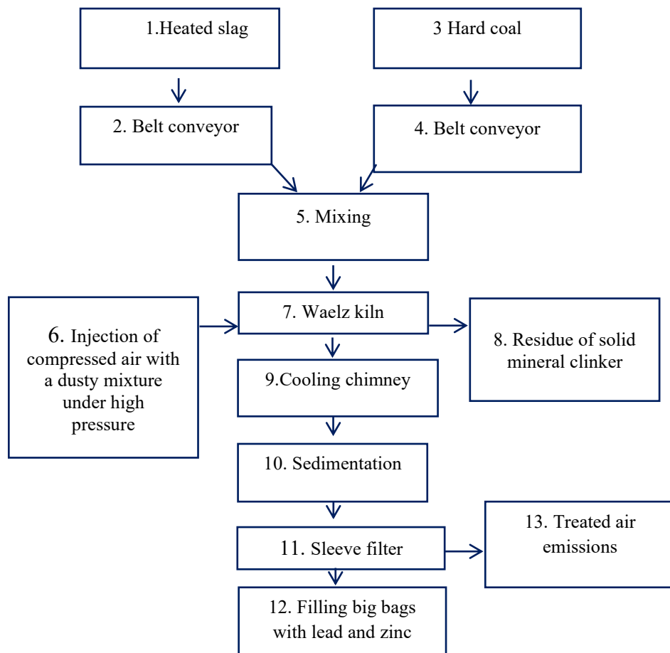
Fig. 3. Technological scheme of the toxic metal extraction method
