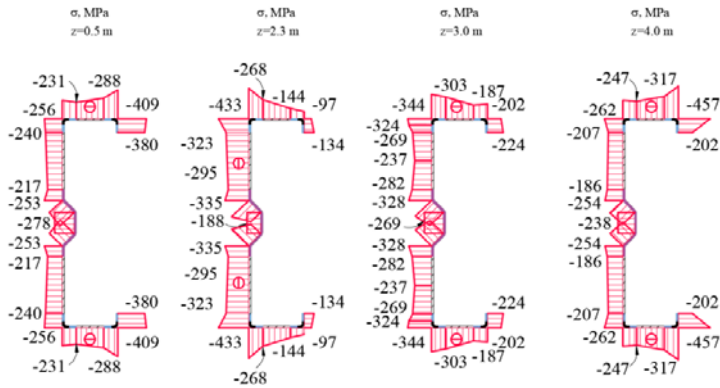
Fig. 10. Stresses in reinforced profile sections
