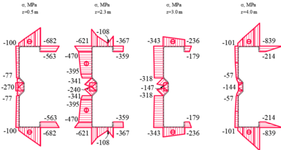
Fig. 7. Stresses in profile sections without reinforcement
