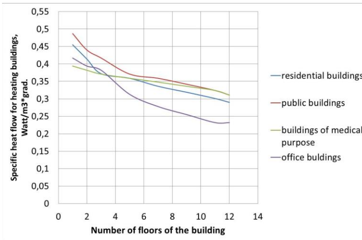
Fig. 2. Diagram of the dependence of the specific heat flow on the heating of buildings according to the data [2].
