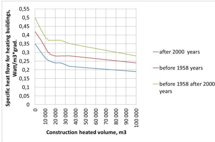
Fig. 1. Diagram of the dependence of the specific heat flow for heating buildings according to data and new data of coefficients a , n .
