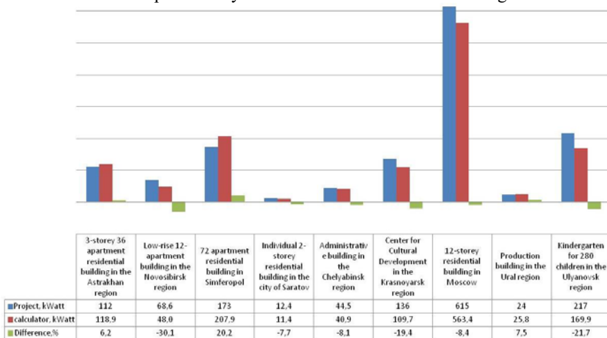
Fig. 3. Trends of the heat flow for heating buildings
