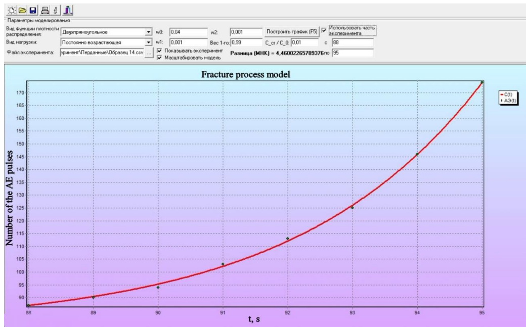
Fig. 5. Screenshot from the programme for modeling the fracture process (red line) and the number of AE pulses (points).
