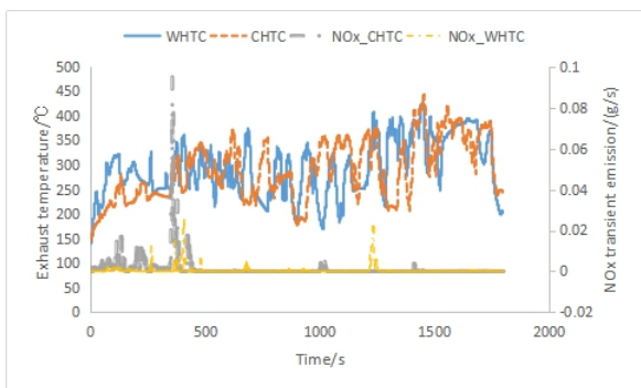
Fig. 12. Exhaust temperature and NOx transient emission of hot CHTC and WHTC.
