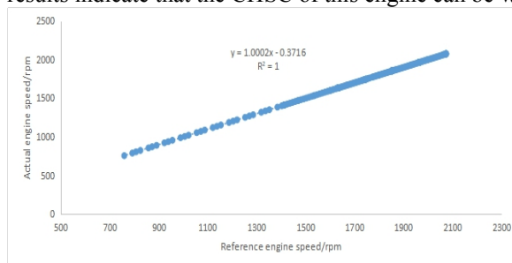
Fig. 2. Engine speed regression analysis of CHSC.
