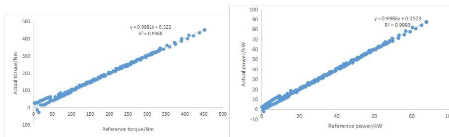
Fig. 3. Engine torque regression analysis of CHSC. Fig. 4. Engine power regression analysis of CHSC.
