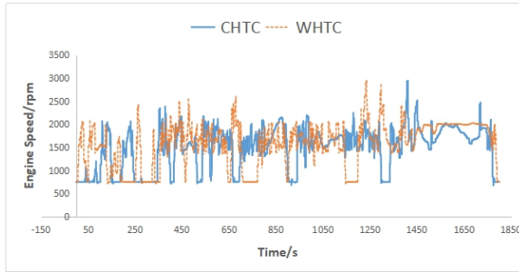
Fig. 5. Engine speed comparison between CHTC and WHTC.
