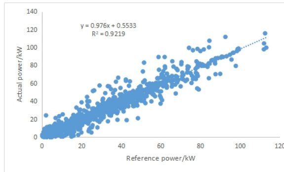
Fig. 10. Engine power regression analysis of CHTC.
