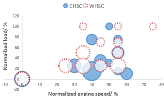
Fig. 1. Operating points comparison of CHSC and WHSC.
