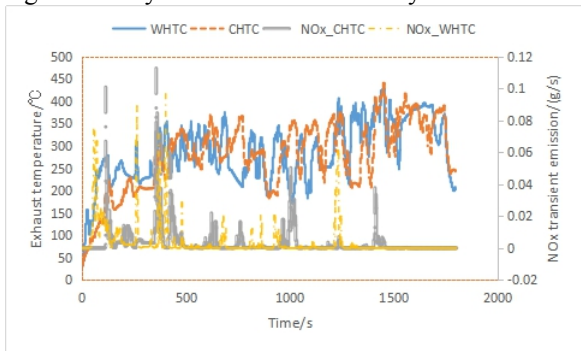
Fig. 11. Exhaust temperature and NOx transient emission of cold CHTC and WHTC.
