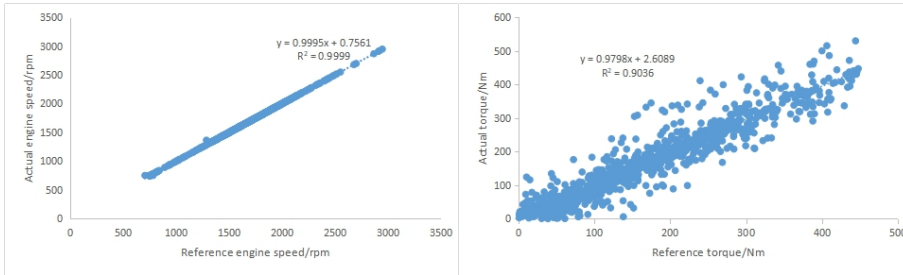
Fig. 8. Engine speed regression analysis of CHTC. Fig. 9. Engine torque regression analysis of CHTC.
