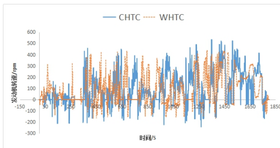
Fig. 6. Engine torque comparison between CHTC and WHTC.
