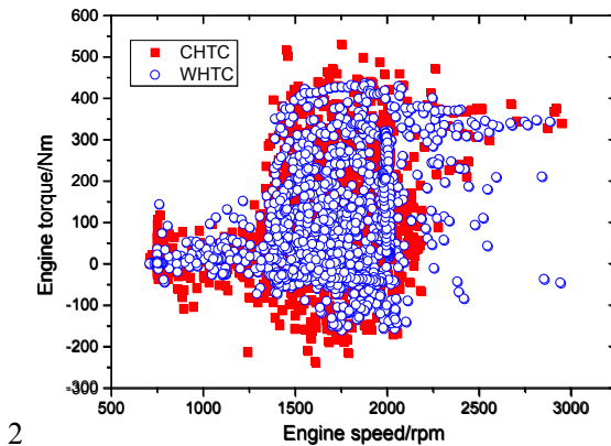
Fig. 7. Engine operating points distribution of CHTC and WHTC.
