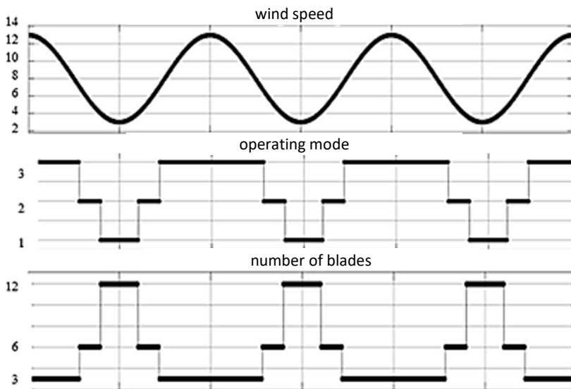
Fig. 5. Graphs of operating modes of WT and wind speeds
