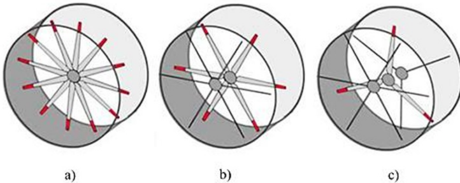
Fig. 1. Modes of CRWT operation at low (a), medium (b) and high (c) wind flow velocities
