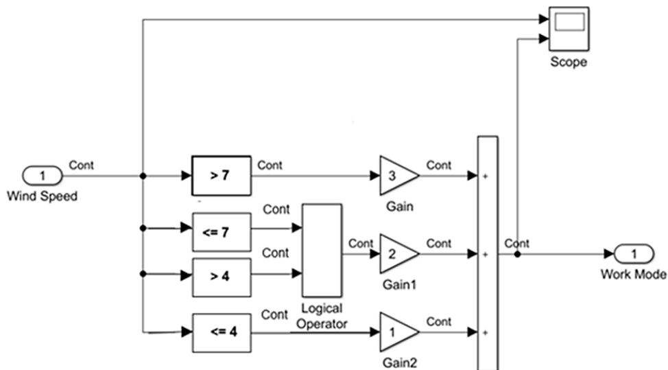
Fig. 4. Diagram of block "Calculation of the generator operating mode"
