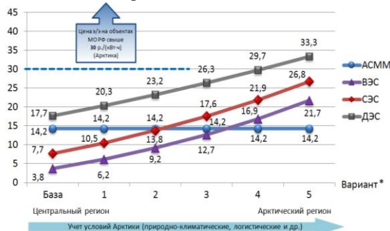
Fig. 3 The cost of electricity generated by SNP, wind, diesel, and solar utilities, depending on natural and logistics conditions
