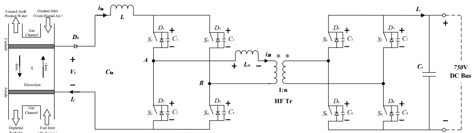
Fig. 2. PEMFC current-fed dual-active full-bridge DC/DC converter.
