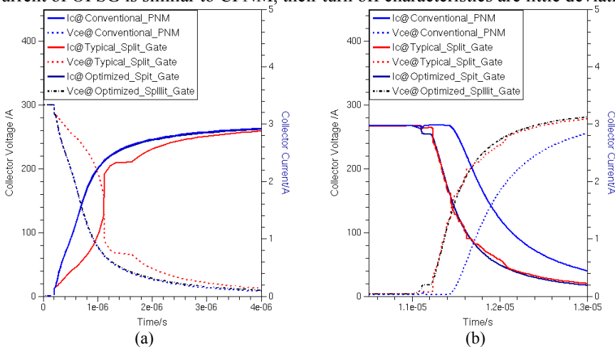
Fig. 6. Comparison of collector current and voltage, (a) during turn-on, (b) during turn-off.
