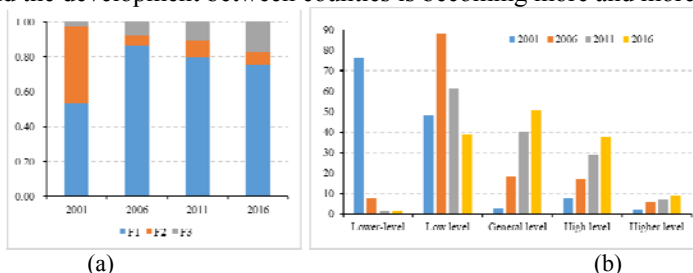
Fig. 2. The change trends of weight of three principal components (a) and number of county units at different levels (b).
