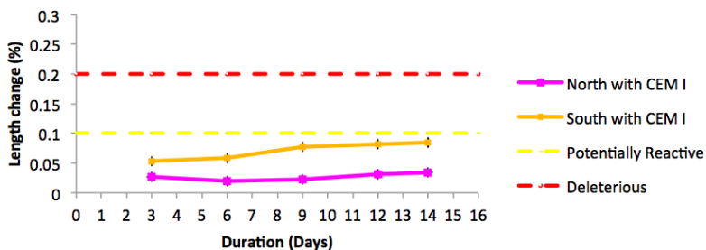
Fig. 1. Length Change Behavior of Mortar Bars Made with CEM I under AAR-2 during 14 days
