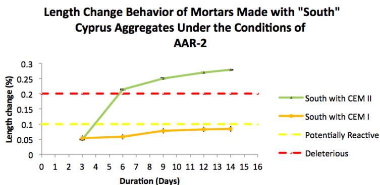
Fig. 3. Length Change Behavior of Mortar Bars Made with "South" Aggregate under AAR-2 during 14 days
