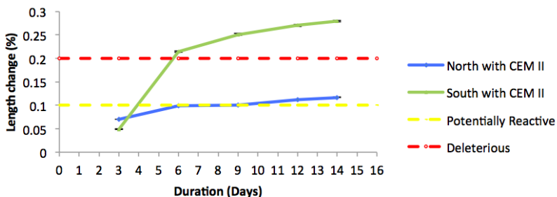
Fig. 2. Length Change Behavior of Mortar Bars Made with CEM II under AAR-2 during 14 days
