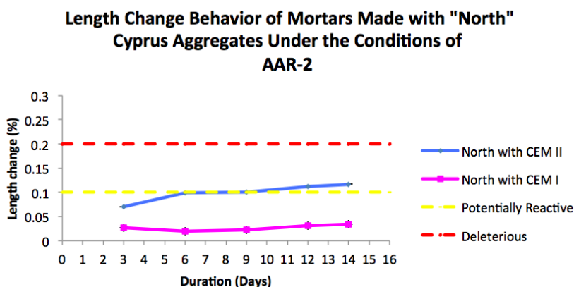
Fig. 4. Length Change Behavior of Mortar Bars Made with "North" Aggregate under AAR-2 Cyprus during 14 days.
