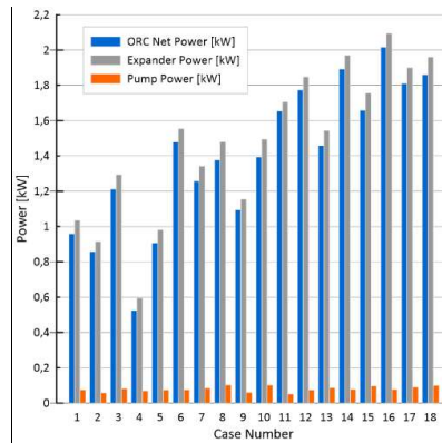
Figure 6 – Recovered power
