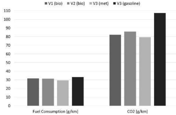
Fig. 2. Comparison of fuel consumption and CO2 emissions during a WLTC driving cycle.
