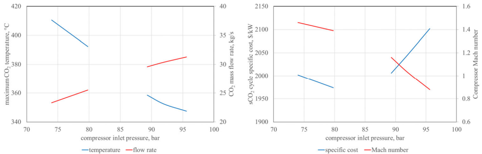
Fig. 4. Maximum cycle temperature, \text{CO}_2 mass flow rate, specific cost and compressor Mach number as functions of the minimum fluid pressure when adopting a compressor with open impeller and vaned diffuser.
