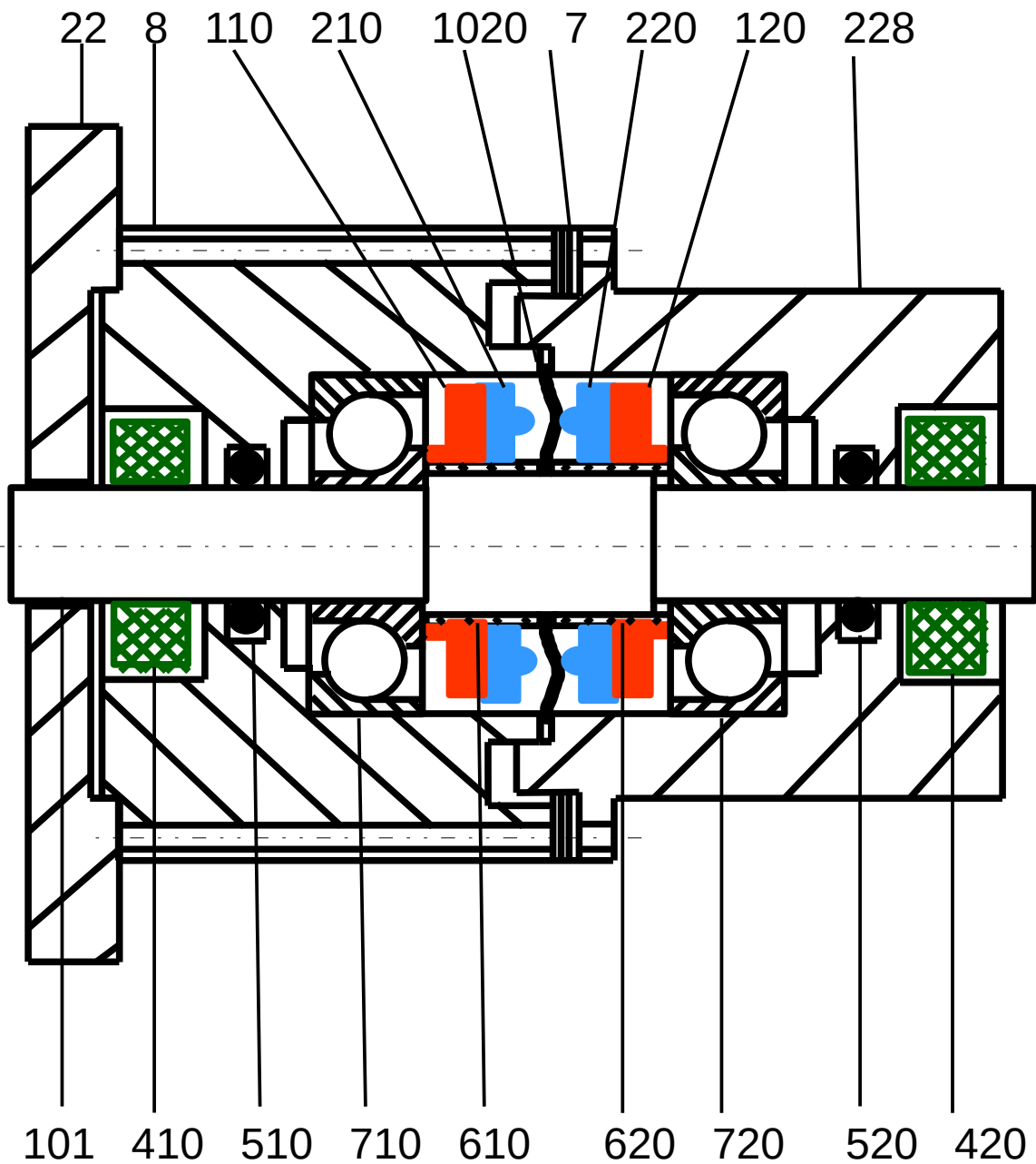
Fig. 1. Twist disk (1020) around alternating shaft (101) enabling absolute sealing
