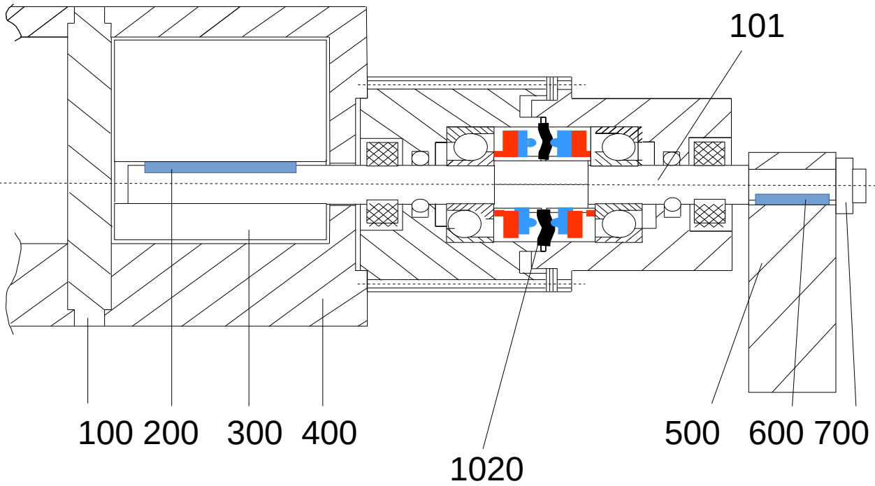
Fig. 2. Twist disk (1020) around alternating shaft (101) enabling absolute sealing for a Stirling-Franchot engine with prismatic “flipper” pistons (300)
