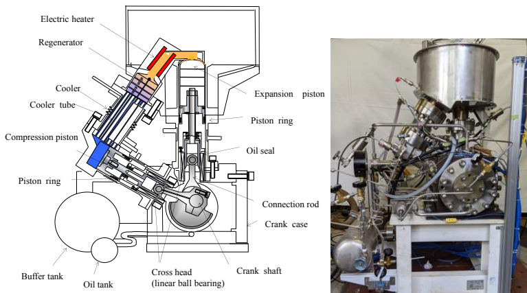
Fig. 1. NS03T engine
