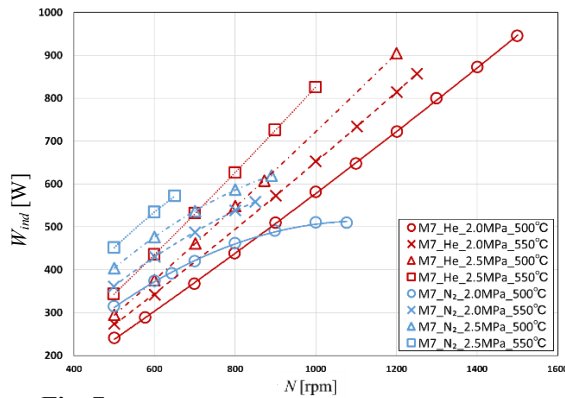
Fig. 7. Indicated power with M7 Mesh sheet
