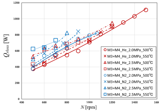
Fig. 14. Regenerator losses in M3+M4 Mesh sheet
