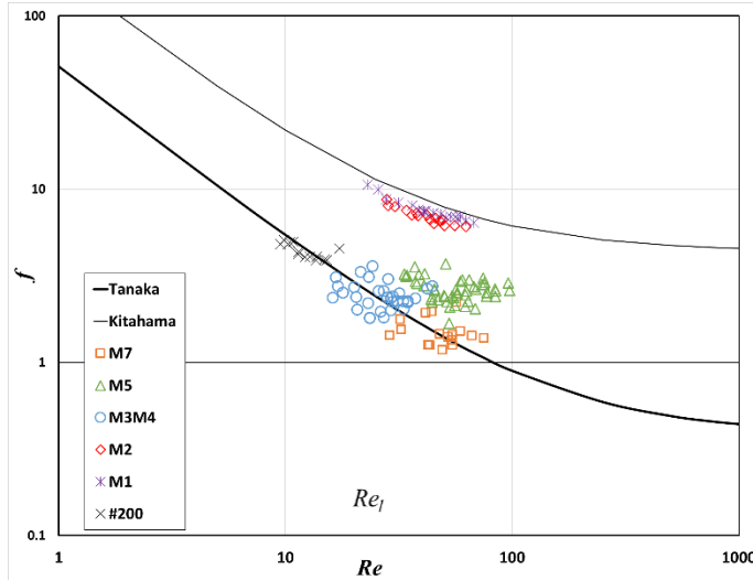
Fig. 17. Friction coefficient with Re
