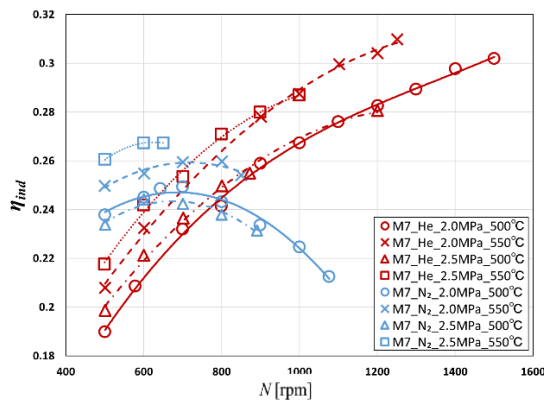
Fig. 10. Indicated efficiency with M7 Mesh sheet
