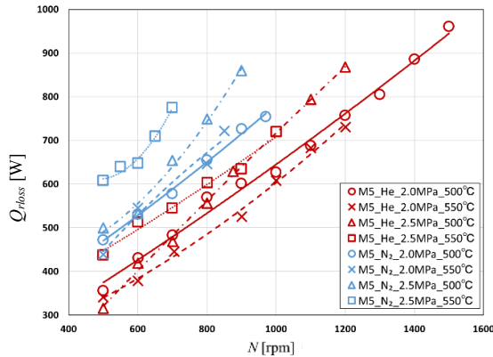
Fig. 15. Regenerator losses in M5 Mesh sheet
