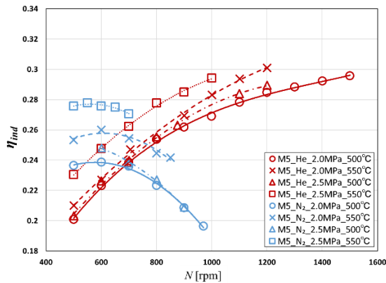
Fig. 9. Indicated efficiency in M5 Mesh sheet
