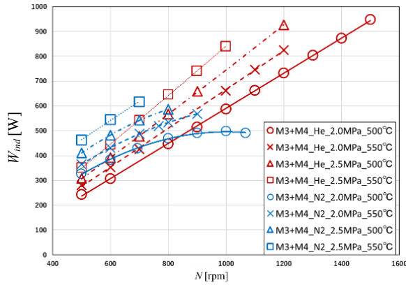
Fig. 5. Indicated power with M3+M4 Mesh sheet
