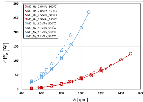
Fig. 13. Pressure loss in M7 Mesh sheet
