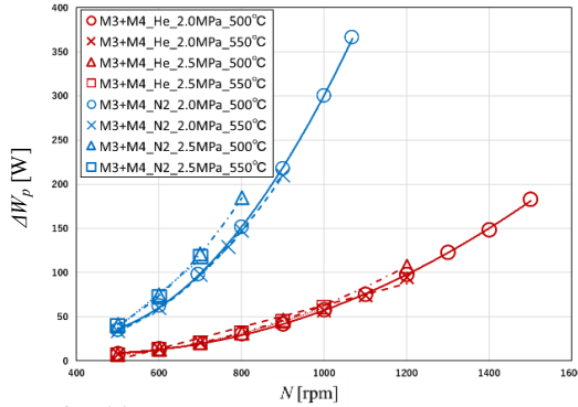
Fig. 11. Pressure loss in M3+M4 Mesh sheet
