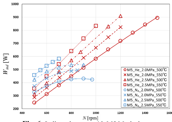
Fig. 6. Indicated power with M5 Mesh sheet
