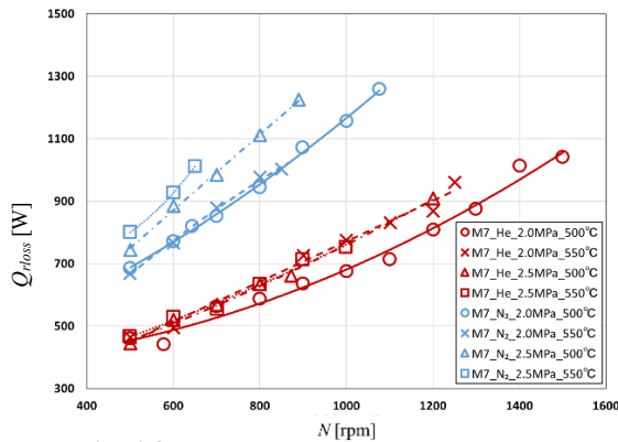
Fig. 16. Regenerator losses in M7 Mesh sheet
