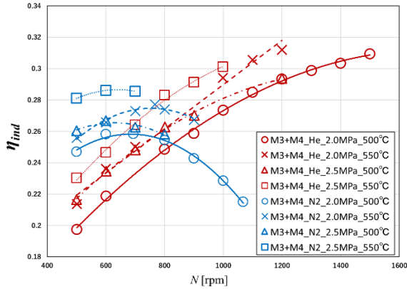
Fig. 8. Indicated efficiency in M3+M4 Mesh sheet
