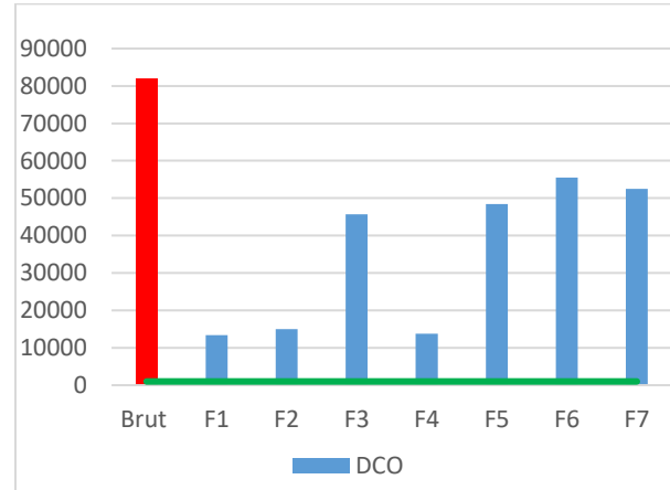
Figure7: Abatement of DCO after treatment in used matrix
