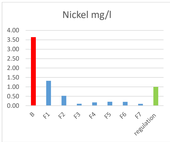
Figure5: Abatement of Nickel after treatment in used matrix
