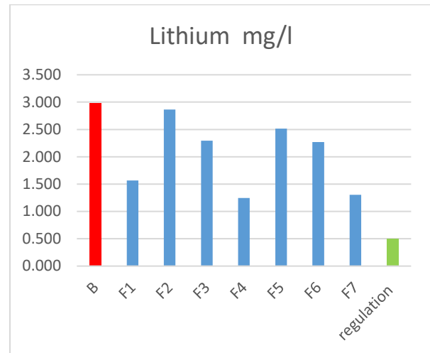
Figure 4: Abatement of Lithium after treatment in used matrix
