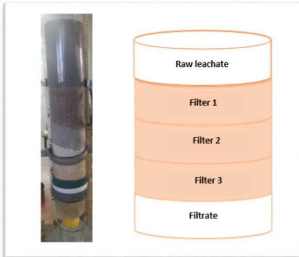
Figure 2: The experimental setup
