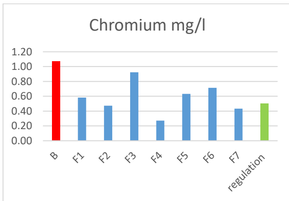
Figure6: Abatement of Chrome after treatment in used matrix
