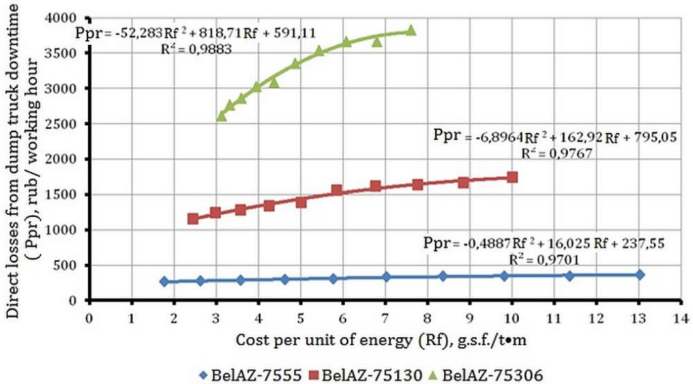
Fig. 5. The relationship between the value of direct losses from downtime of open-pit vehicles and specific energy costs
