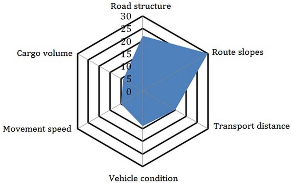
Fig. 2. The influence of operation of technical and technological factors on the energy intensity of transportation (percentage)
