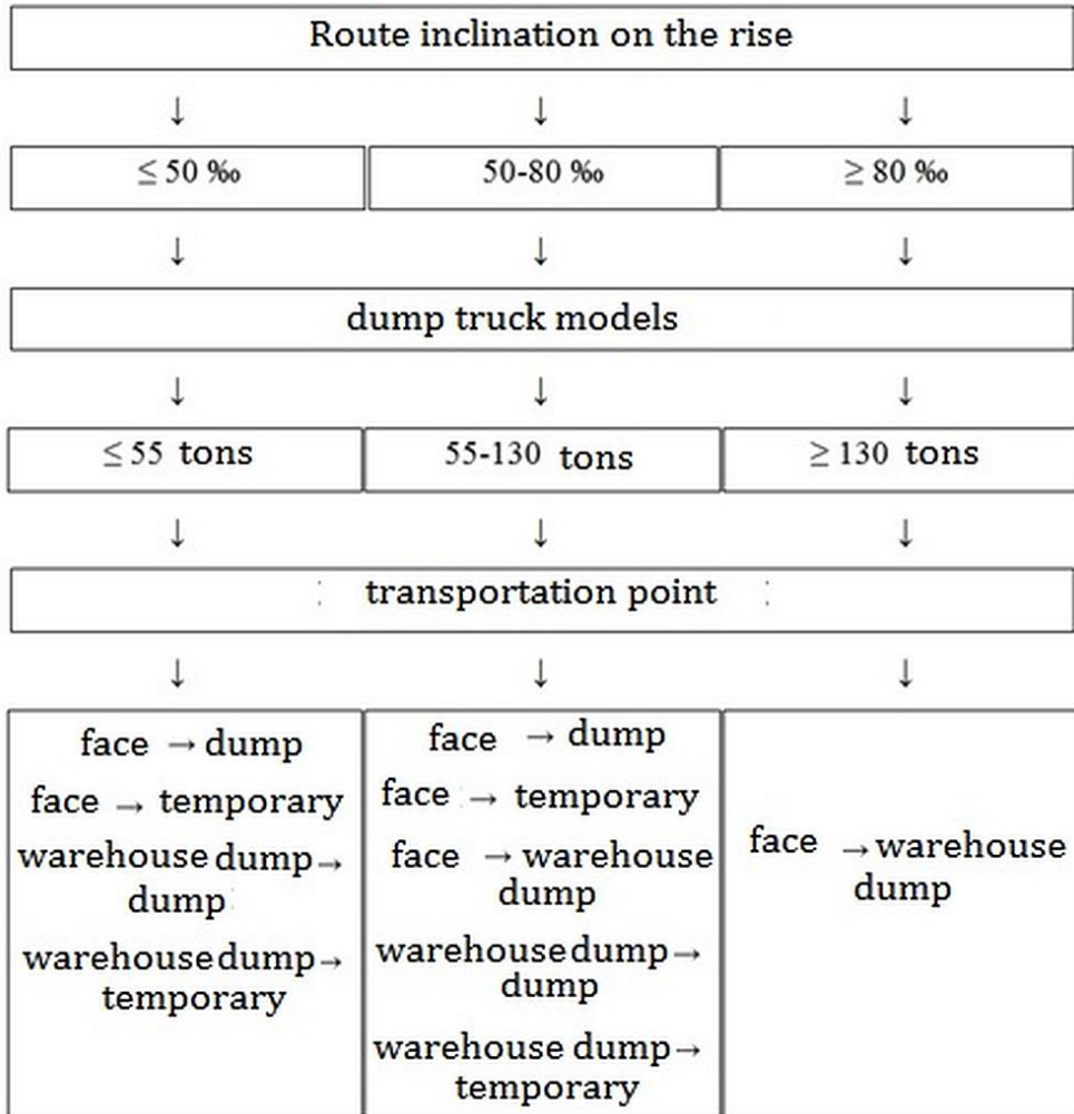
Fig. 3. The scheme of distribution of dump trucks of different load capacities depending on the slope of the route on the rise
