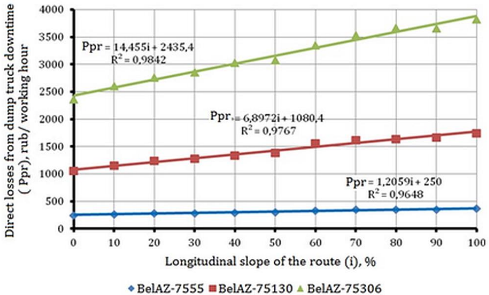
Fig. 4. The influence of the value of the longitudinal slope of the route on the change in direct losses from downtime of open-pit vehicles
