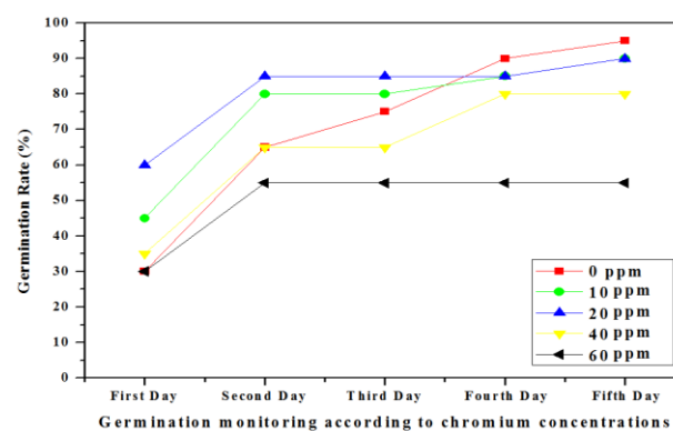
Fig. 1 Germination rate of radish seeds exposure to Chromium
