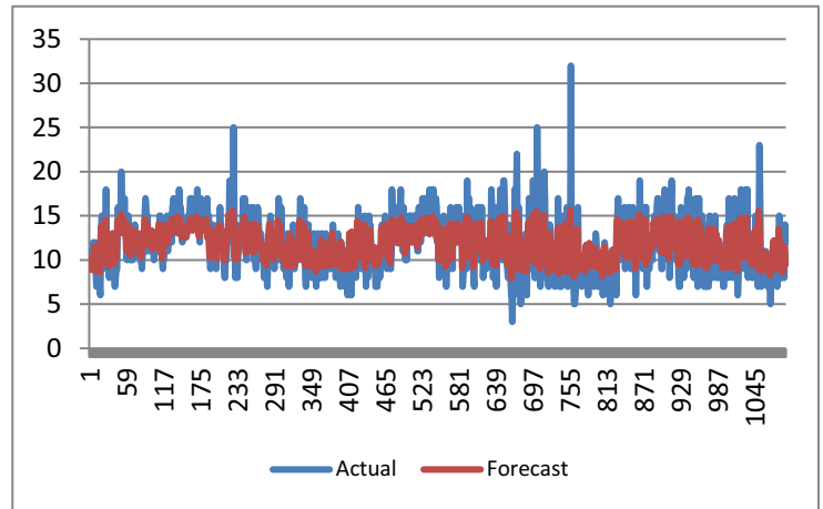
Fig. 4. The actual wind speed series and the series estimated by NARX-P
