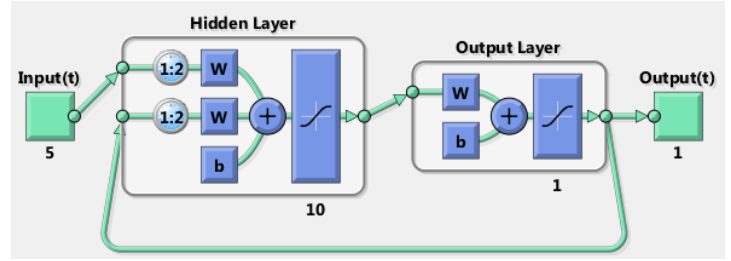
Fig. 3. NARX Neural Network – 10 Neurons – Tansig function activation
