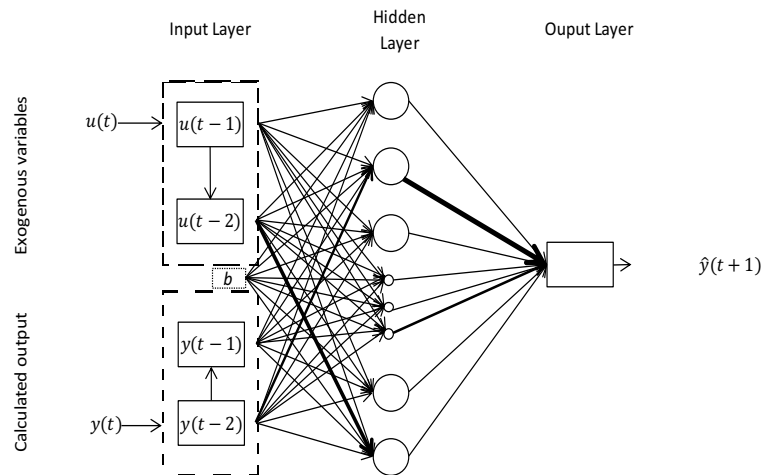
Fig. 5. NARX-SP Representation (18, 10, 1)
