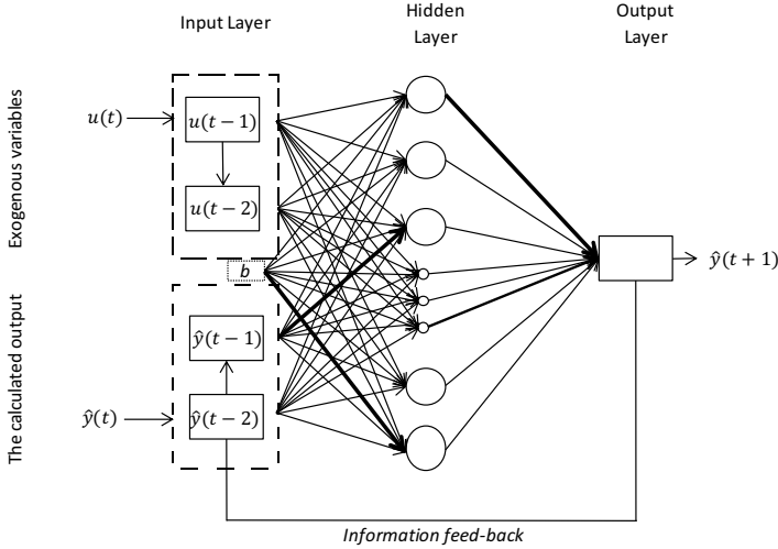
Fig. 2. NARX-P Representation (18, 10, 1)
