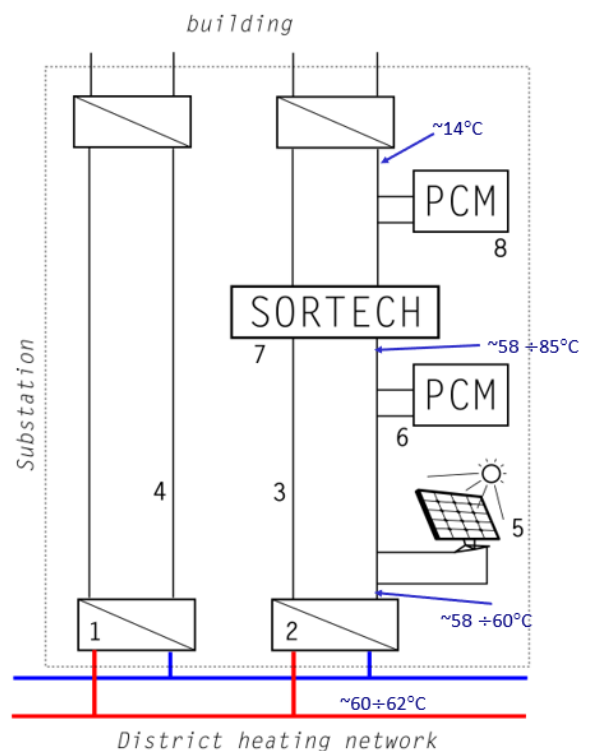
Fig. 2. Simplified scheme of the composite substation
