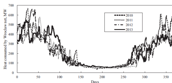
Fig. 1. Yearly profile of heat consumption in a middle-sized Polish city, by Chorowski [4]
