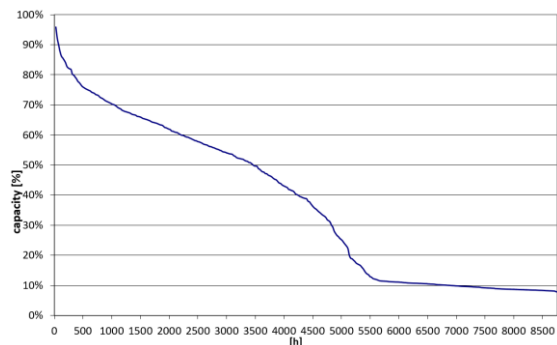
Fig. 5 Annual heat load duration curve
