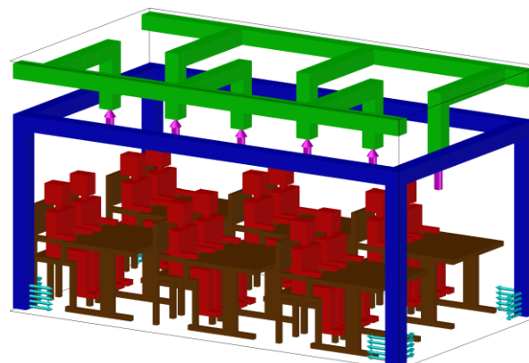
Fig. 1. Scheme of the virtual chamber, equipped with a ventilation system (extraction in green and insufflation in dark blue), the inlet in light blue arrows and outlet in purple arrows, desks (brown) and manikins (red), used in the CFD.
