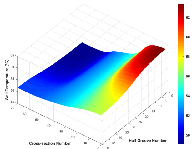
Fig. 8. Temperature distribution through FGHP under localized heat source and sink
