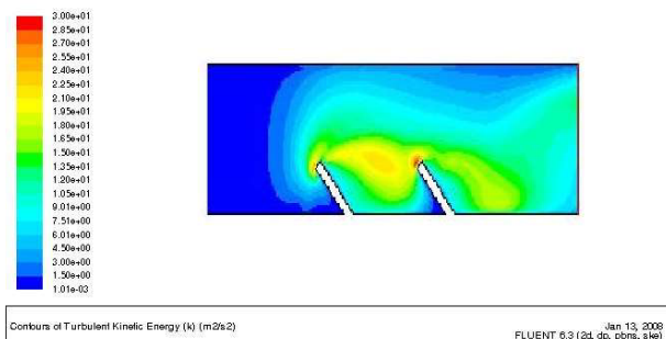
Fig. 17 Turbulent kinetic energy Contour for U inlet 10 m/s (Reynolds = 148 641 )
