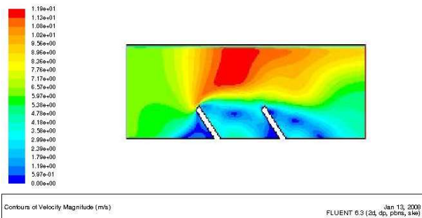
Fig. 5 Velocity Contour for U inlet= 6 m/s (Reynolds =89 072)
