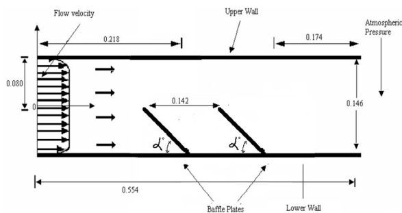
Fig. 1. Geometry of study
