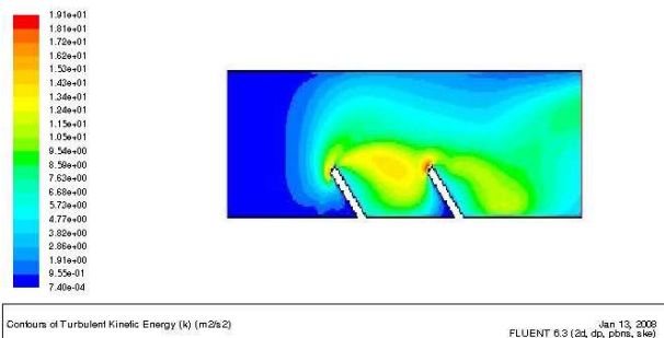
Fig. 15 Turbulent kinetic energy Contour for U inlet= 8 m/s (Reynolds = 118 837 )
