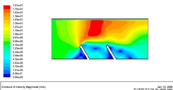
Fig. 9 Velocity Contour for U inlet= 9 m/s (Reynolds = 133 718 )
