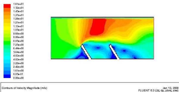
Fig. 8 Velocity Contour for U inlet= 8 m/s (Reynolds = 118 837 )
