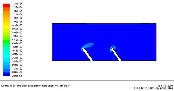
Fig. 20 Turbulent dissipation Contour for U inlet= 6 m/s (Reynolds =89 072)
