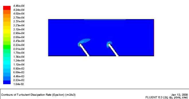
Fig. 23 Turbulent dissipation Contour for U inlet= 9 m/s (Reynolds = 133 718 )
