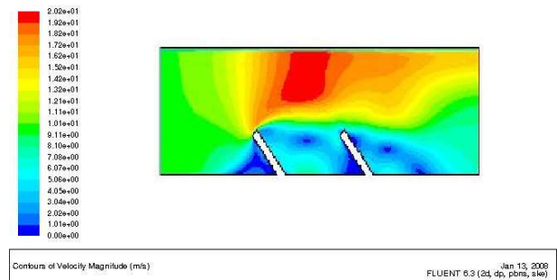
Fig. 10 Velocity Contour for U inlet= 10 m/s (Reynolds = 148 641)
