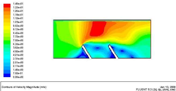
Fig. 6 Velocity Contour for U inlet= 7 m/s (Reynolds = 103 945 )
