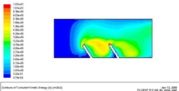
Fig. 13 Turbulent kinetic energy Contour for U inlet= 6 m/s (Reynolds =89 072)
