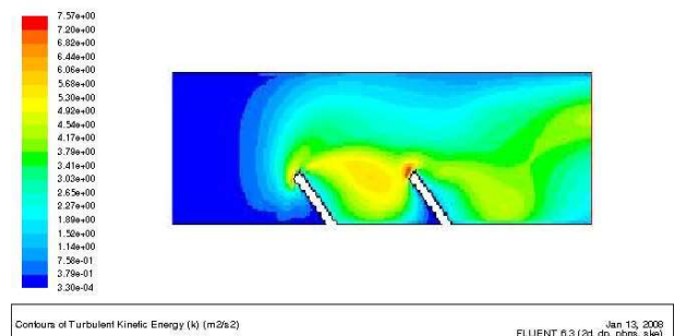
Fig. 12 Turbulent kinetic energy Contour for U inlet= 5 m/s (Reynolds = 74 182)
