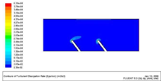
Fig. 24 Turbulent dissipation Contour for U inlet= 10 m/s (Reynolds = 148 641 )
