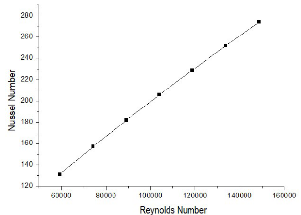
Fig. 25 Nusselt Number profile
