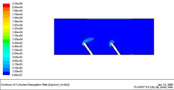
Fig. 21 Turbulent dissipation Contour for U inlet= 7 m/s (Reynolds = 103 945 )
