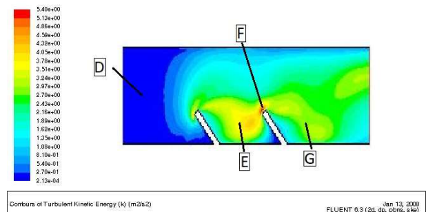
Fig. 11 Turbulent kinetic energy Contour for U inlet= 4 m/s (Reynolds=59346)
