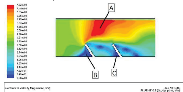
Fig. 3 Velocity Contour for U inlet= 4 m/s (Reynolds=59346)
