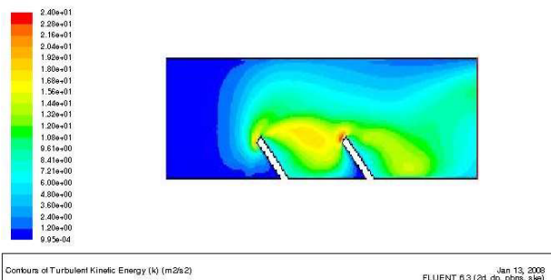
Fig. 16 Turbulent kinetic energy Contour for U inlet= 9 m/s (Reynolds = 133 718 )
