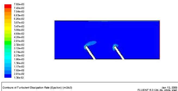
Fig. 19 Turbulent dissipation Contour for U inlet= 5 m/s (Reynolds = 74 182)
