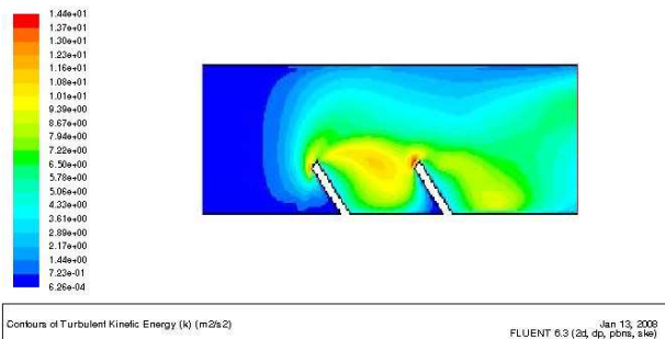
Fig. 14 Turbulent kinetic energy Contour for U inlet= 7 m/s (Reynolds = 103 945 )
