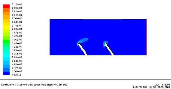
Fig. 22 Turbulent dissipation Contour for U inlet= 8 m/s (Reynolds = 118 837 )
