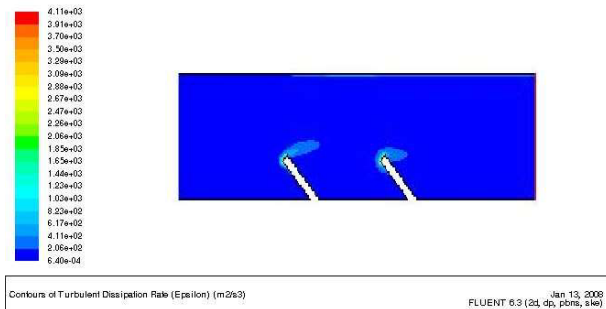
Fig. 18 Turbulent dissipation Contour for U inlet= 4 m/s (Reynolds=59 346)
