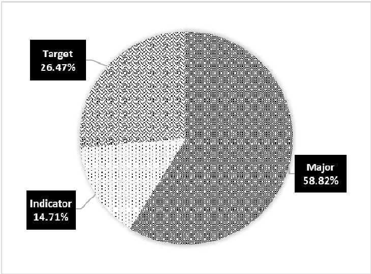
Fig. 4. Fish group composition.
