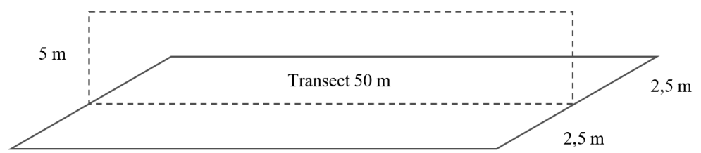
Fig. 2. Survey area dimension by UVC method.
