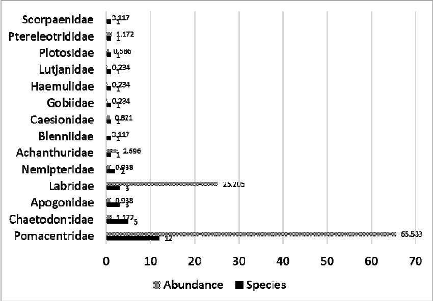
Fig. 3. Fish family comparison in Celukan Bawang area.
