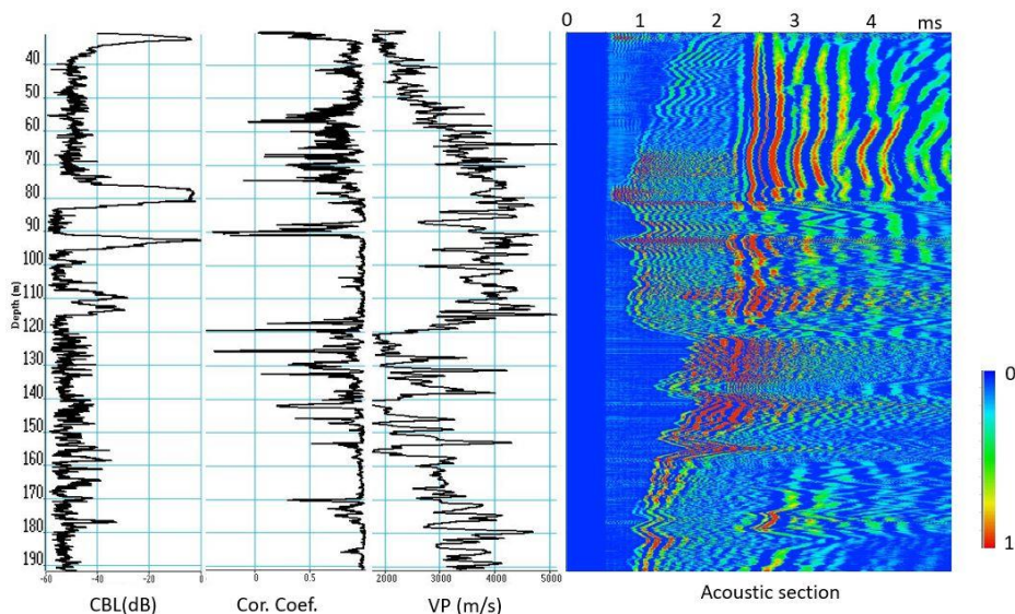
Fig. 5. Acoustic logs and full wave form composite acoustic section. After [1].
