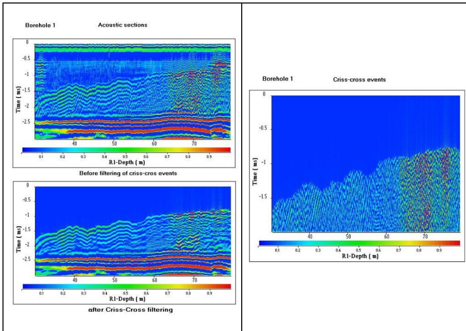
Fig. 6. Acoustic sections recorded in borehole B1
