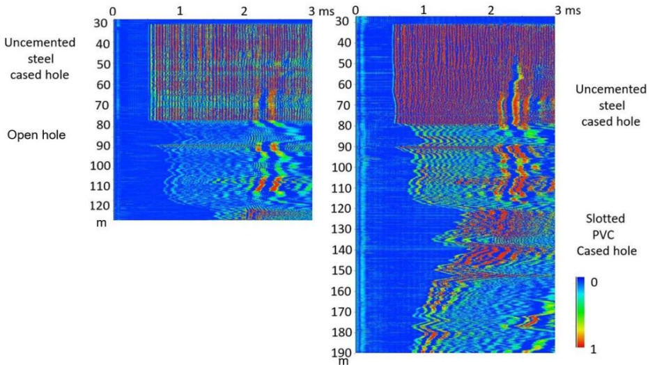
Fig. 4. Acoustic sections in borehole B2 (phases 1 and 2)
