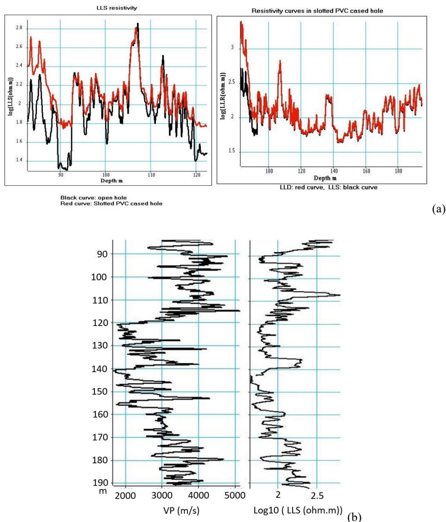
Fig. 15. Resistivity logs after tubing joint filtering in borehole B2 (slotted PVC cased hole): (a) comparison between LLS log in open hole and in slotted PVC cased hole, comparison between LLS and LLD logs in slotted PVC cased hole. (b) comparison between acoustic velocity log and resistivity log (LLS)
