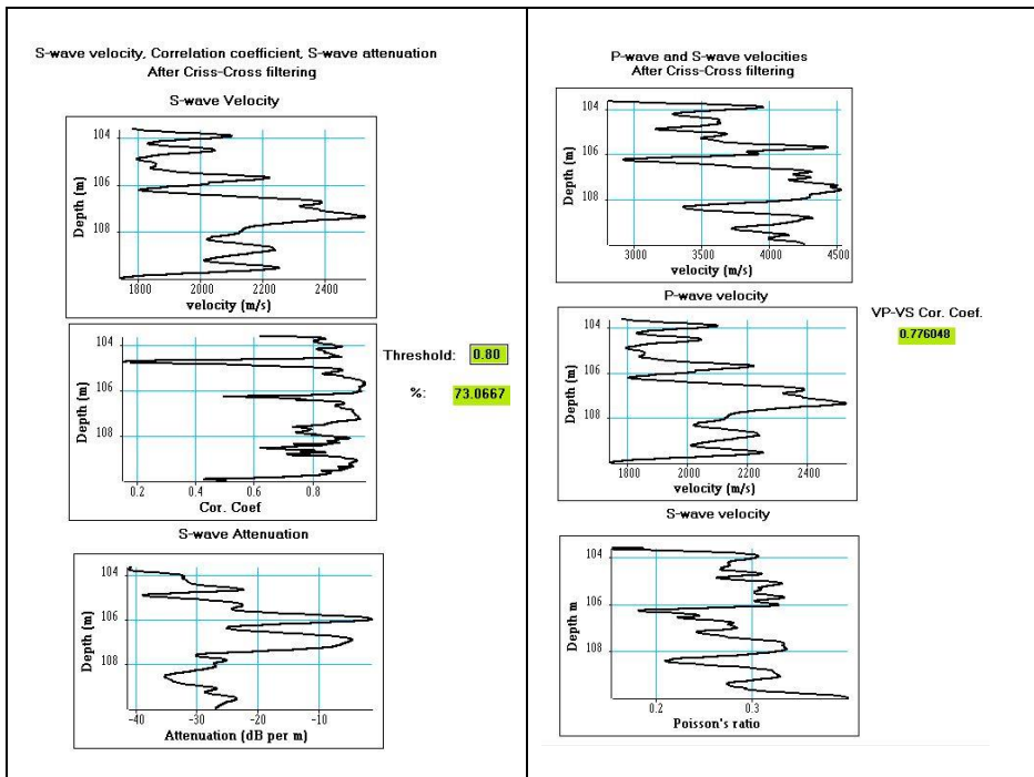
Fig. 10. S-wave acoustic logs in borehole B2 (open hole)
