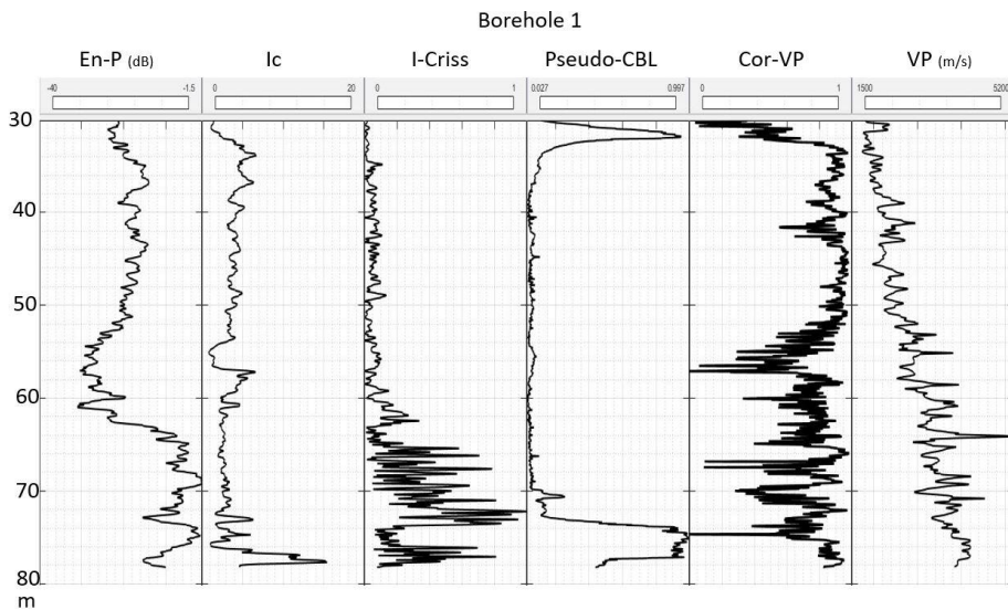
Fig. 7. Acoustic logs in borehole B1
