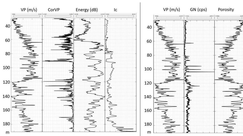
Fig. 12. Acoustic logs (VP, Cor-VP, Energy, I_c , Porosity) and Gamma ray (GN)
