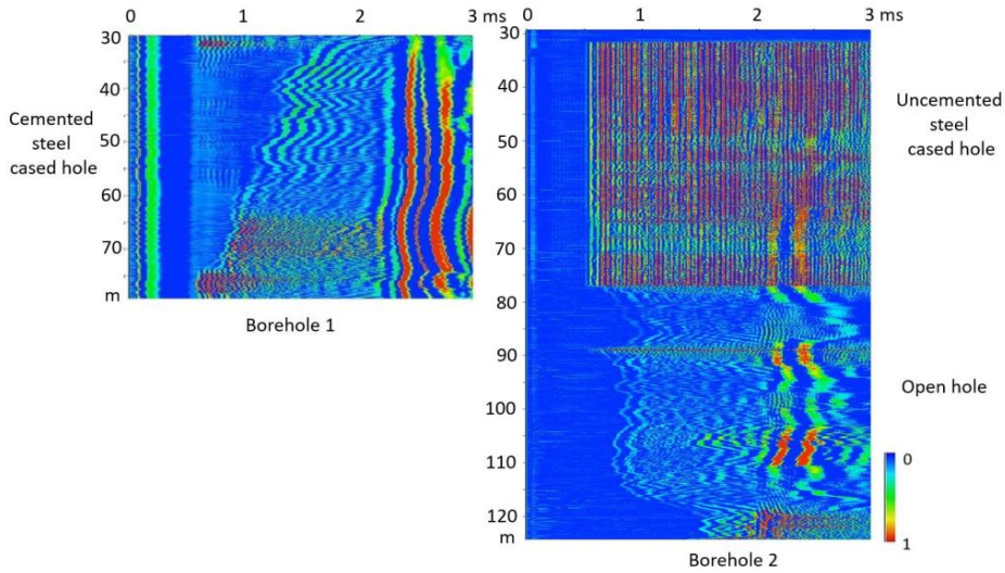
Fig. 3. Acoustic sections in boreholes B1 and B2 (phase 1).
