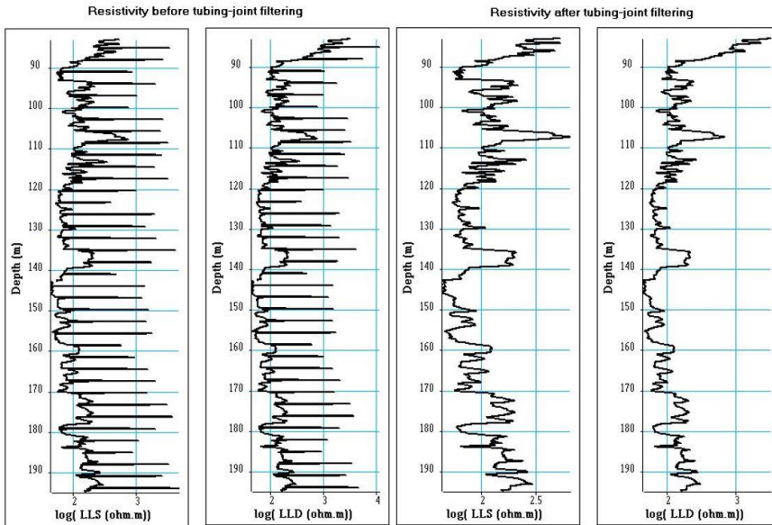
Fig. 14. Resistivity logs in borehole B2 (slotted PVC cased hole)
