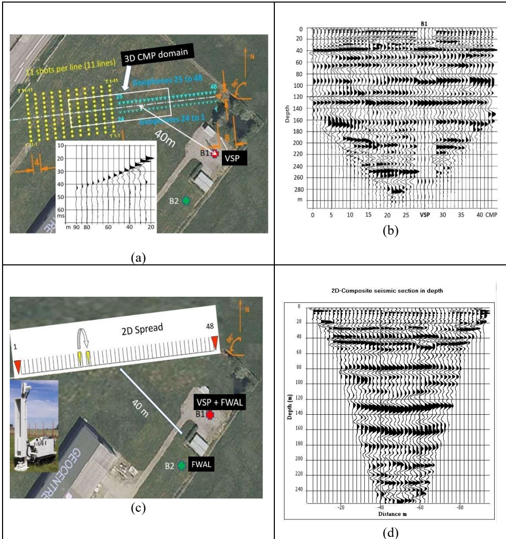
Fig. 2. Seismic imaging: (a) 3D seismic spread, borehole locations (B1 and B2), VSP recorded in B1, (b) 3D composite inline section in depth after calibration by VSP corridor stacked trace, (c) 2D seismic spread and view of the seismic source, (d) 2D composite section in depth. After [1]
