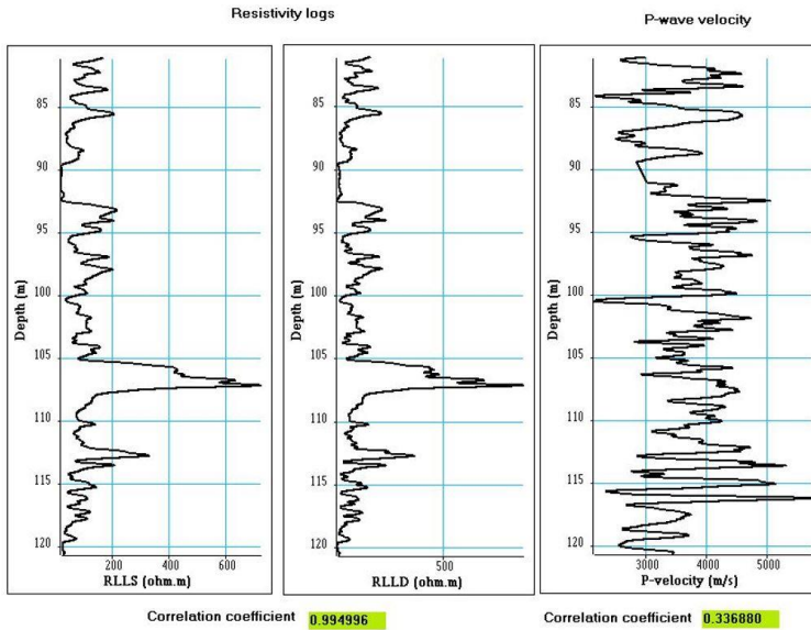
Fig. 13. Resistivity logs (LLS, LLD) and acoustic velocity in borehole B2 (open hole)
