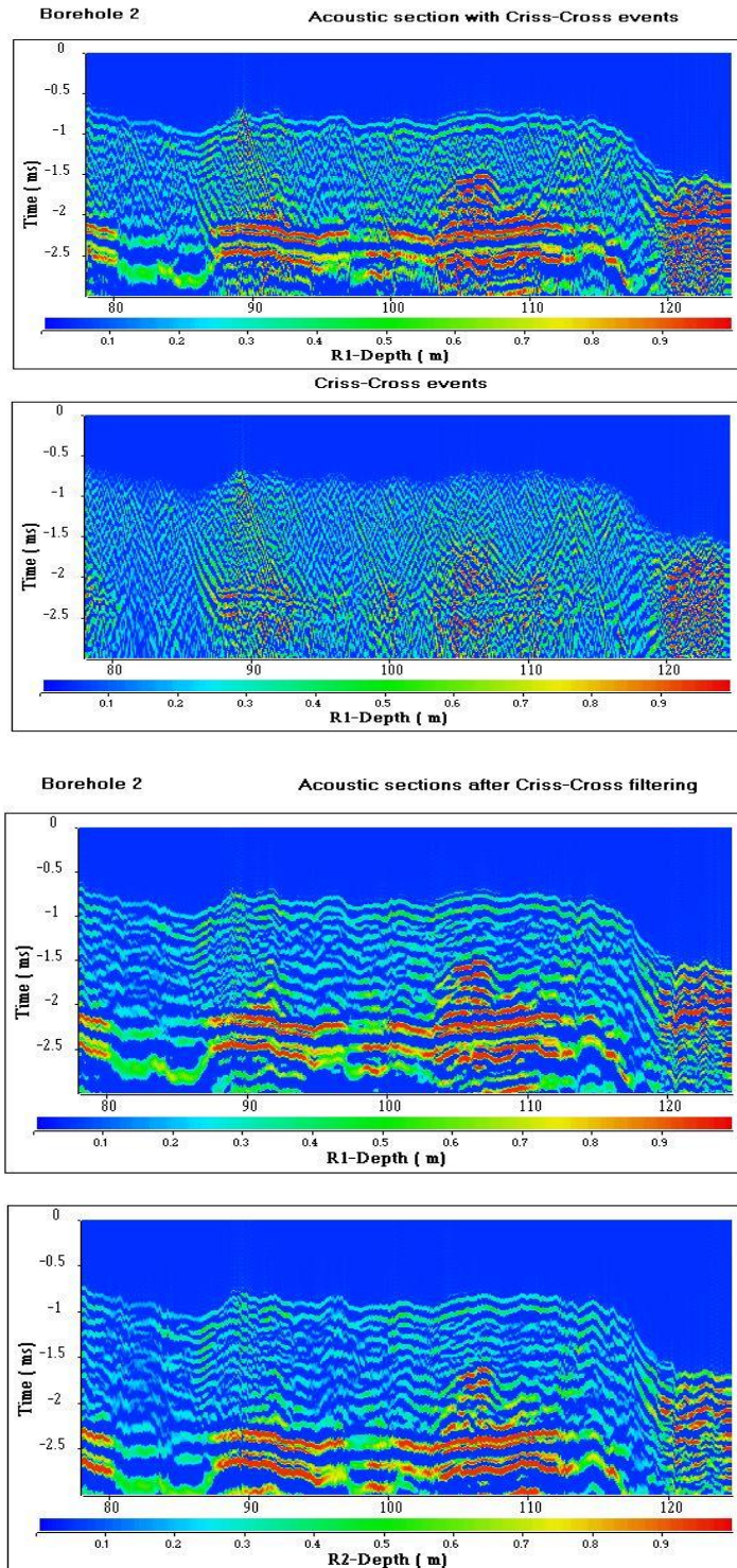
Fig. 8. Acoustic sections recorded in borehole B2 (open hole)
