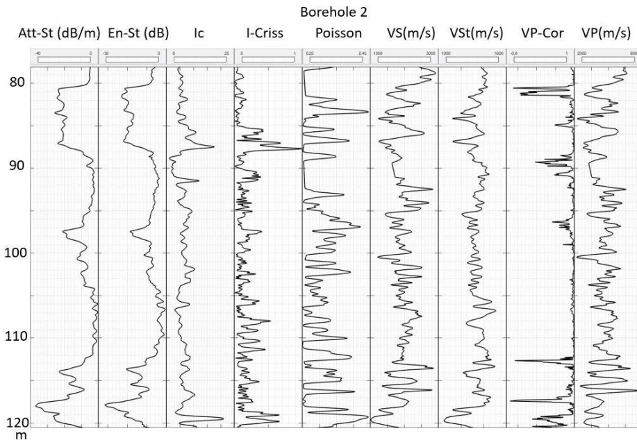
Fig. 11. Acoustic logs for mechanical studies in borehole B2 (open hole)
