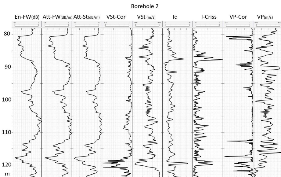
Fig. 9. Acoustic logs in borehole B2 (open hole)
