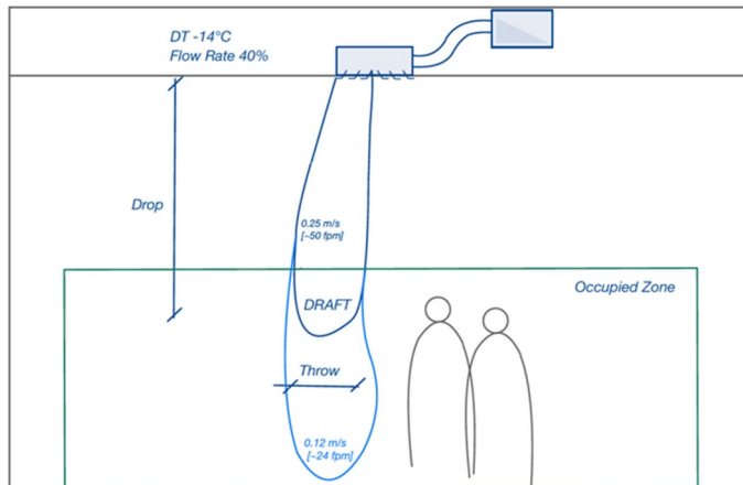
Fig. 2c. Behaviour of a diffuser in cooling mode, constant \Delta T , flow at 40% of the rated value.
