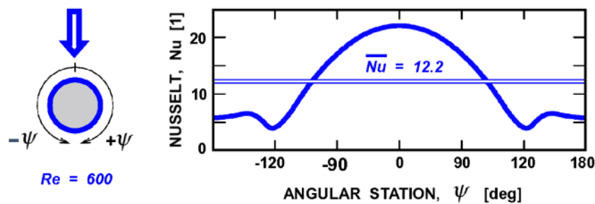
Fig. 5. Distribution of local Nusselt number on a cylinder in cross flow
