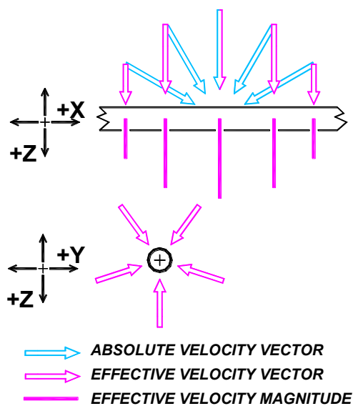
Fig. 4. Relation between absolute and effective flow velocities
