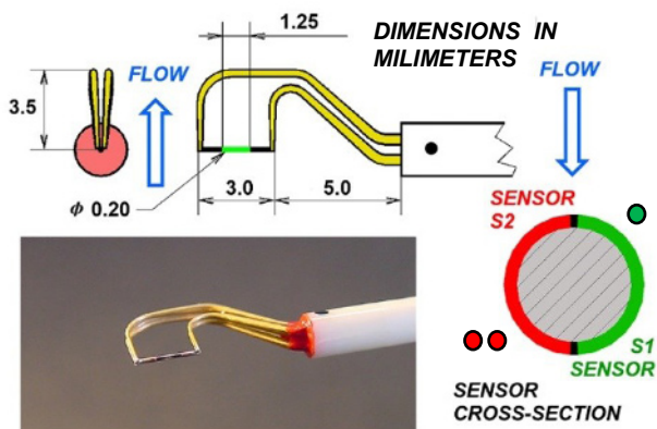
Fig. 3. Split-fiber thermo-anemometer probe
