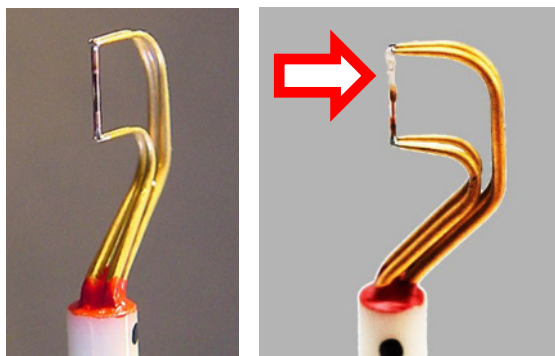
Fig. 13. View of clean and contaminated split-fiber probe
