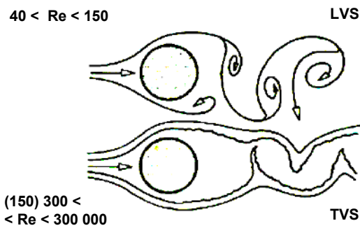
Fig. 12. Flow Reynolds number effects on fiber wake vortex street (LVS = laminar vortex street, TVS = turbulent vortex street) [11]
