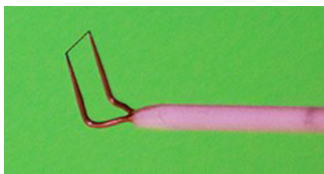
Fig. 2. Right-angle cylindrical fiber thermo-anemometer probe
