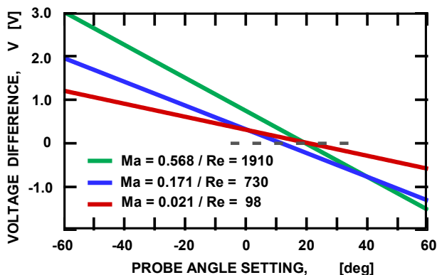
Fig. 8. Spread of effective zero incidence angles
