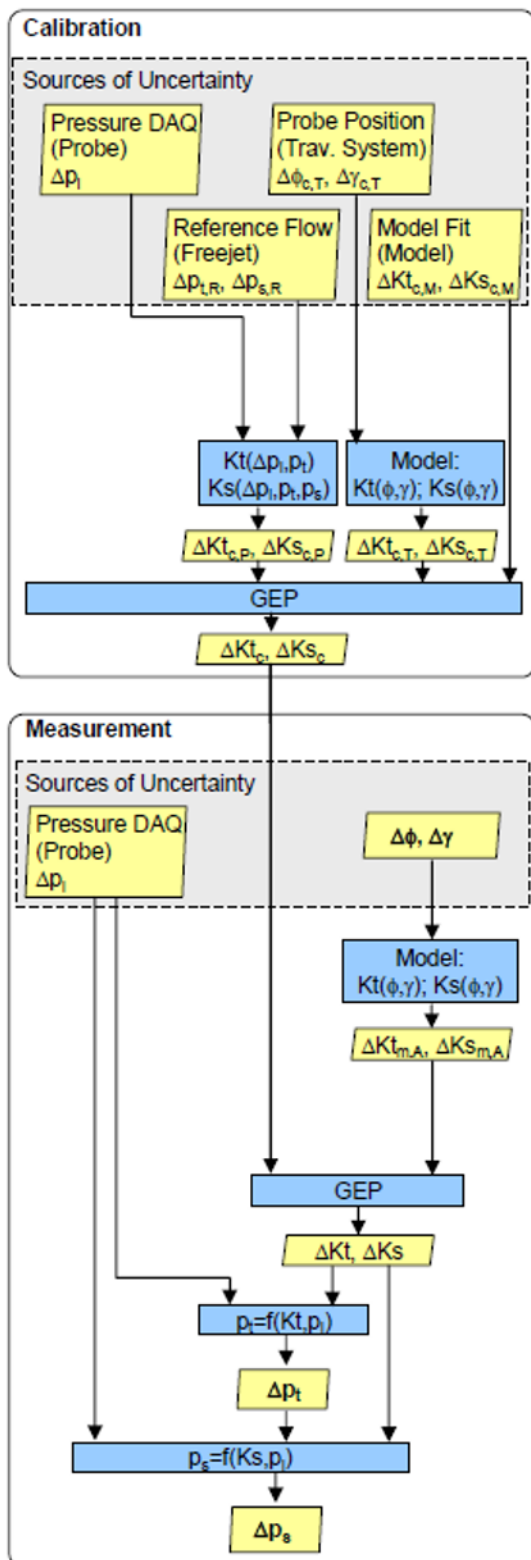
Fig. 11. Uncertainty propagation of total and static pressure measurement – Method A
