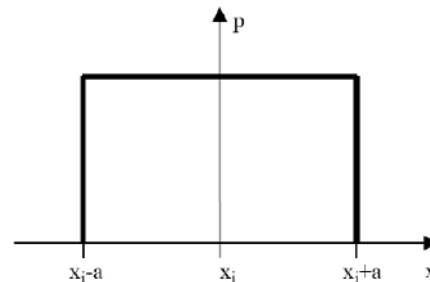
Fig. 1. Rectangular distribution
