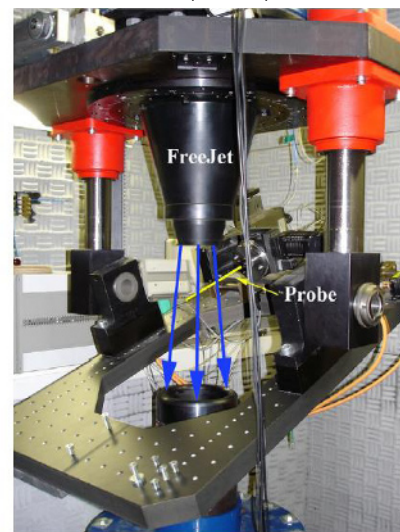
Fig. 4. Freejet probe calibration facility
