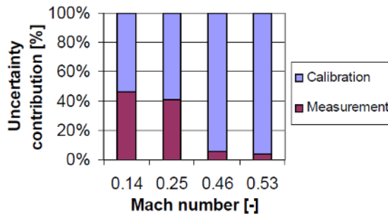
Fig. 8. Uncertainty contribution of calibration and measurement of four Mach numbers [-] (using Calibration polynoms)
