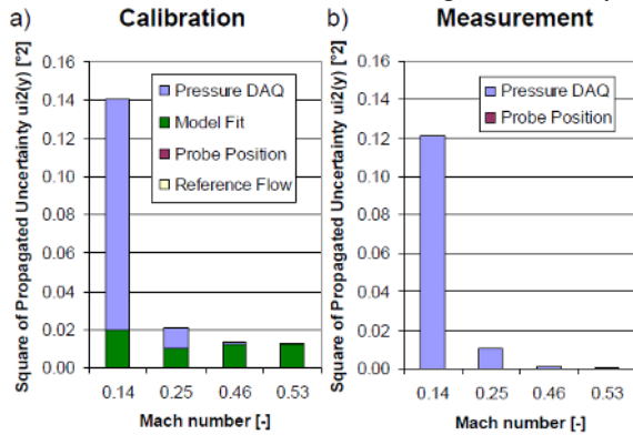
Fig. 7. Square of propagated uncertainties u_i^2(y) [ ^\circ^2 ] of four Mach numbers [-] a) Calibration b) Measurement (using Calibration polynoms)
