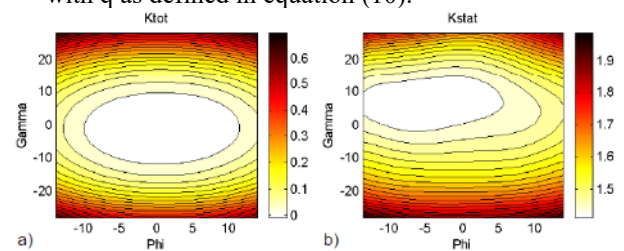
Fig. 10. Distribution of calibration coefficients with respect to yaw and pitch angles at Ma = 0.25 , a) K_t , b) K_s
