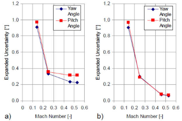
Fig. 9. Expanded uncertainty ( k=2 ) of the yaw and pitch angle derived with a) Calibration polynoms b) Look-up tables
