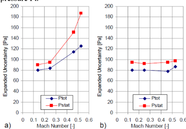
Fig. 13. Expanded uncertainty ( k=2 ) of the total pressure and static pressure derived with a) Calibration Polynoms b) Look-up tables
