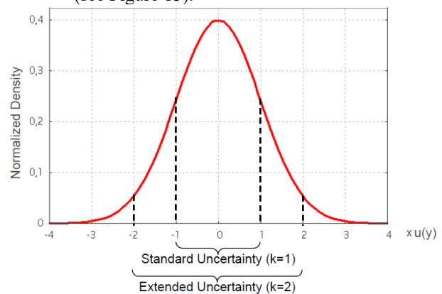
Fig. 15. Normalized normal distribution of uncertainty u(y) with marked range of standard and extended uncertainty
