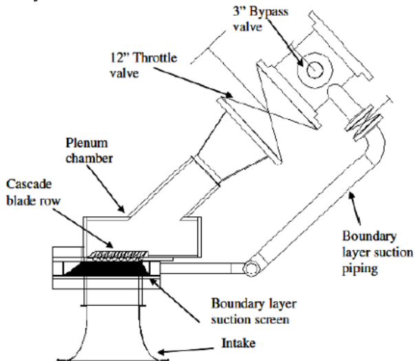
Fig. 3. Layout of the experimental facility
