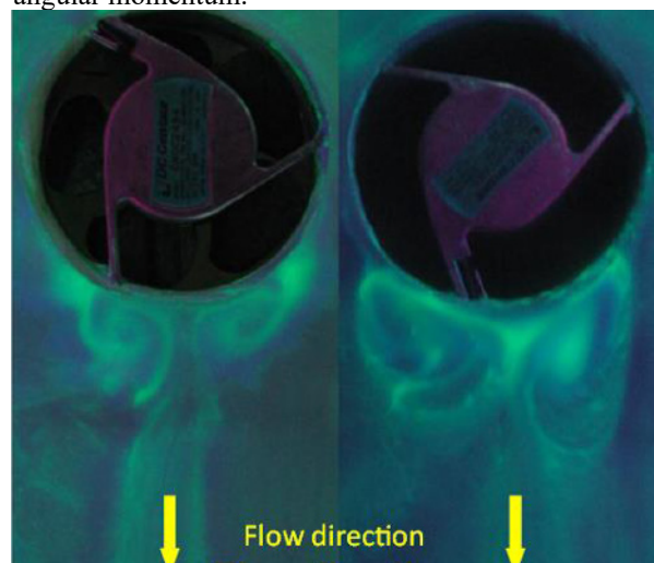
Fig. 1. Hanging Vortices at the trailing edge of the fan for very low viscosity of the paint mixture
