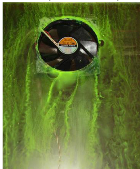
Fig. 6. Proper and roughcast paint mixture and the effect of UV light on picture quality a) waves and b) bubbles at the wake of the fan, due to separation between white spirit and mixture.
