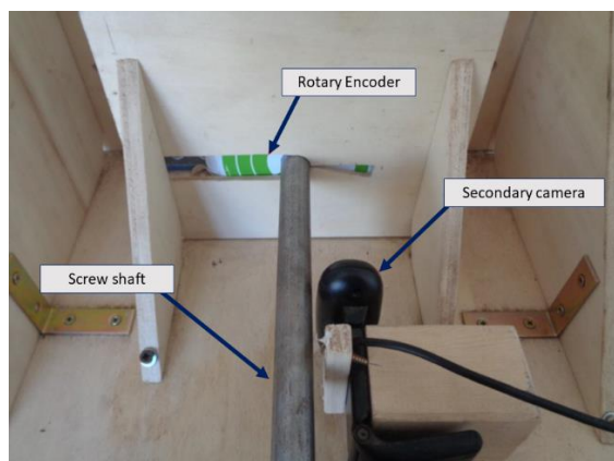
(a) Turn number acquisition system
