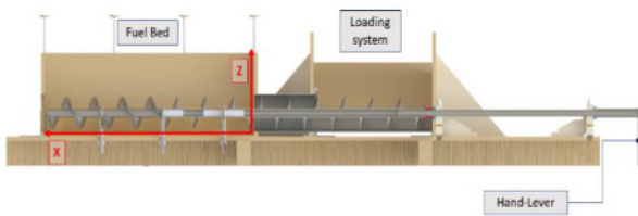
(b) Side view render of the setup
