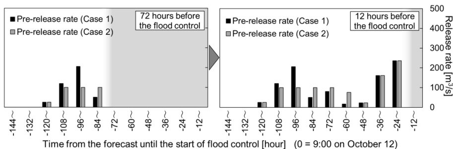
Fig. 9.b. Calculations of pre-release volume and rates - Pre-release rate at each interval.
