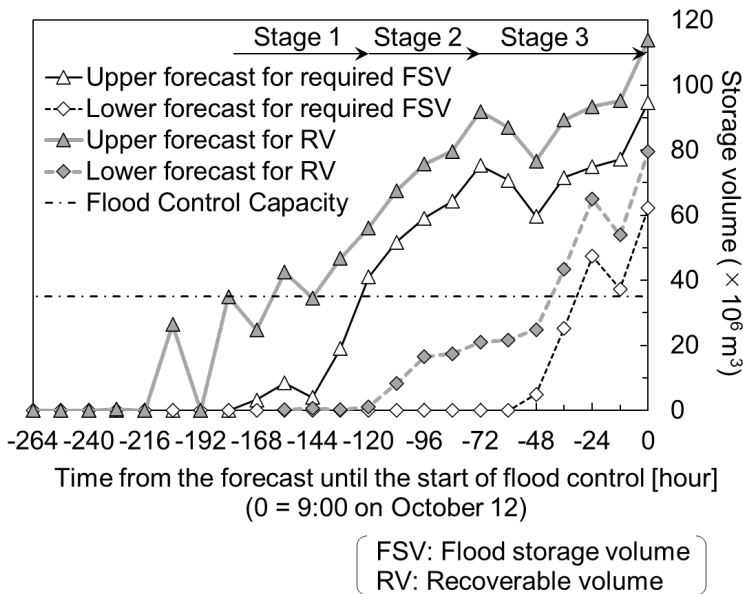
Fig. 7. Changes in required flood storage volume and recoverable volume.
