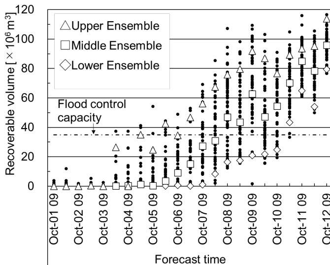
Fig. 6. Changes in recoverable volume.
