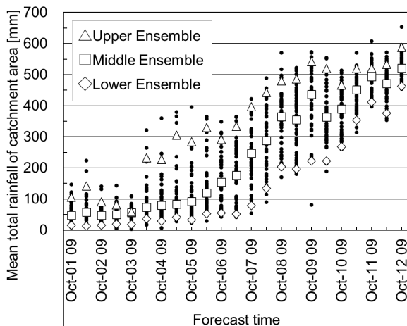
Fig. 3. Changes in mean total rainfall of model dam catchment area.
