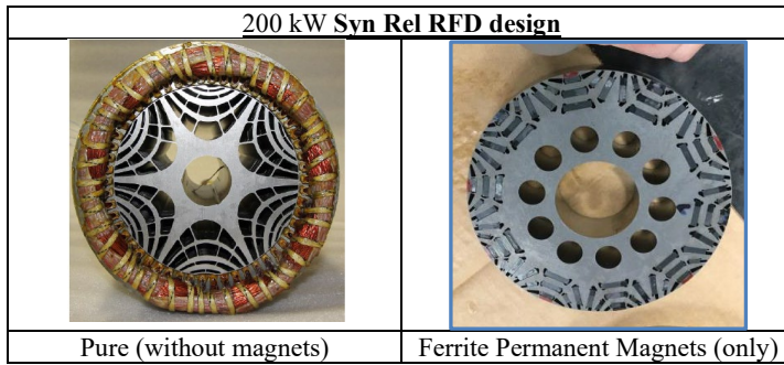
Figure 3: RFD SynRel designs without magnets and with ferrite permanent magnets
