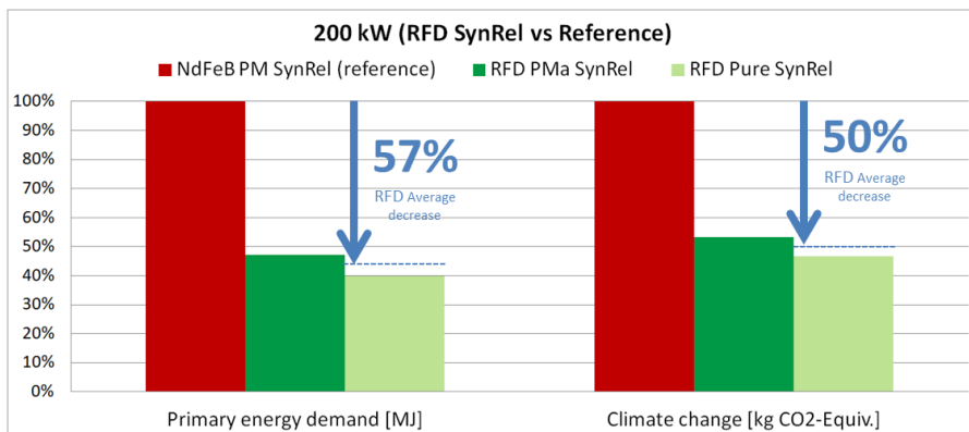
Figure 5: Environmental Impact comparison of REFREEDRIVE motors with “PM-assisted” and “pure ferrite” against current automotive electric motor (NdFeB permanent magnets SynRel)
