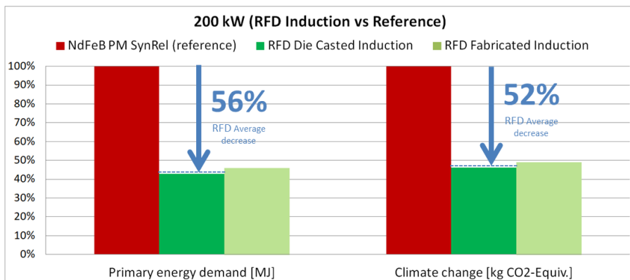
Figure 6: Environmental Impact comparison of REFREEDRIVE induction motors with copper against current automotive electric motor (NdFeB permanent magnets SynRel)
