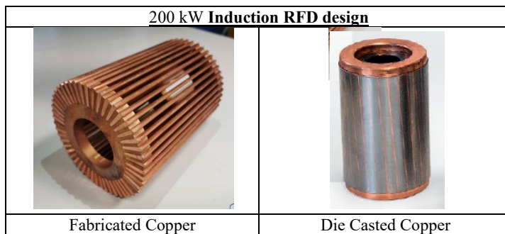
Figure 2: RFD Induction rotor designs with copper
