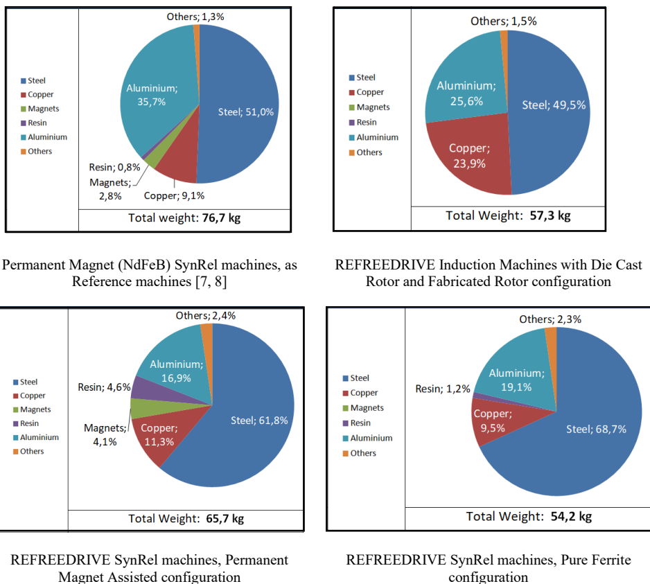
Figure 4: Mass configuration of different electrical machines
