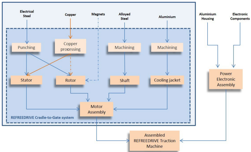
Figure 1: System Boundaries for the REFREEDRIVE Life Cycle Assessment
