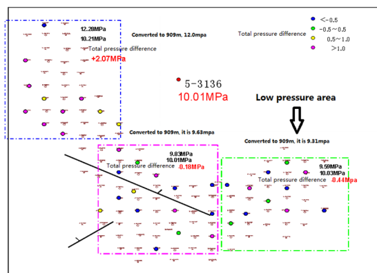
Fig. 6 Pressure distribution of block
