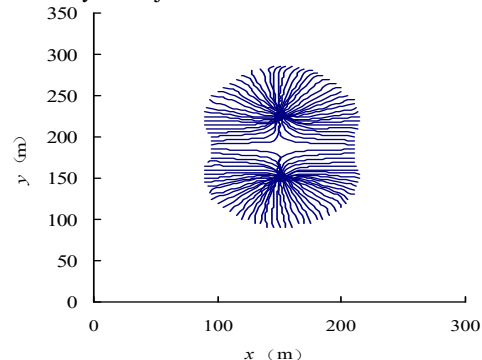
(b) Polymer injection in Juba well for 3 months
