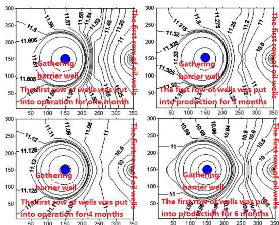
Fig. 5 Distribution diagram of formation pressure field in the first row of wells outside the accumulation barrier at different production times
