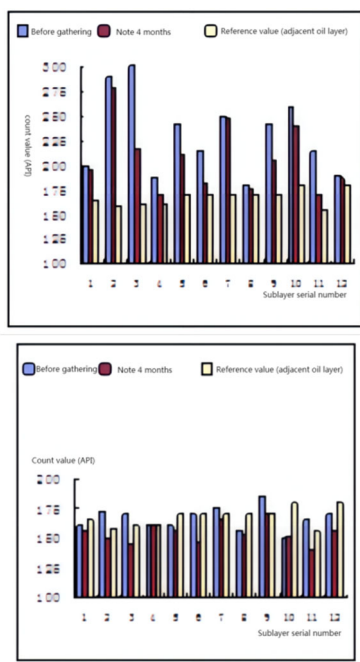
Fig. 1 Test results of thick layer counting of neutron-neutron monitoring wells in barrier band
