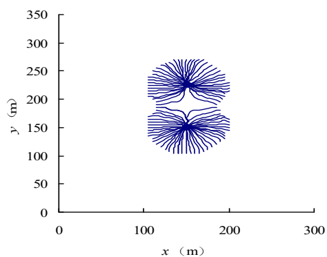
(a) Polymer injection in the barrier well for 2 months
