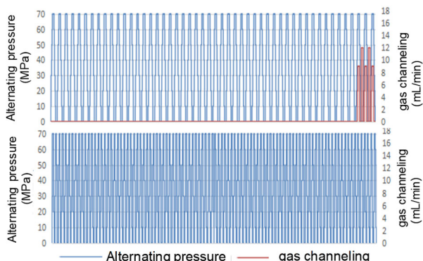
Fig. 2 Channeling flow of conventional cement and toughened cement at 105 °C and alternating stress of 70 MPa( \rho=1.90\text{g/cm}^3 )
