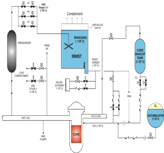
Figure 1: PXS passive core cooling system diagram
