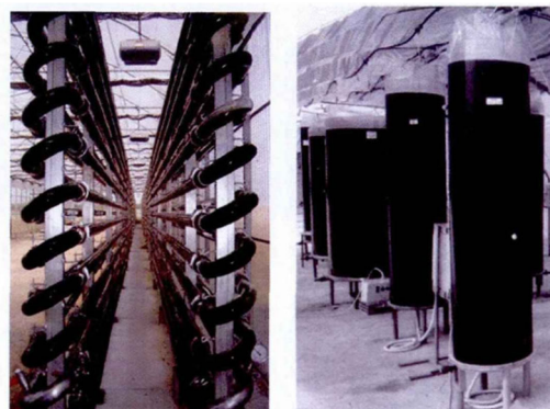
Figure 1 Tubular photobioreactor and column photobioreactor
