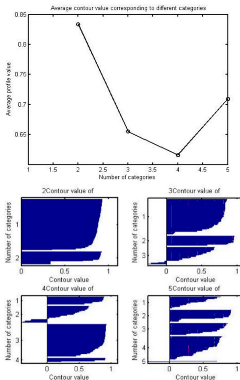
Figure 2: Clustering Analysis for the Original Data & Number of Categories Vs. i -th Contour Value of Clustering
