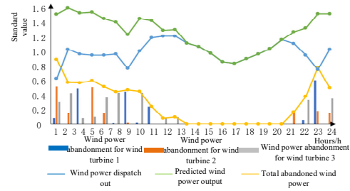
Fig.1 Wind power forecast output and unit combination model to dispatch wind power output
